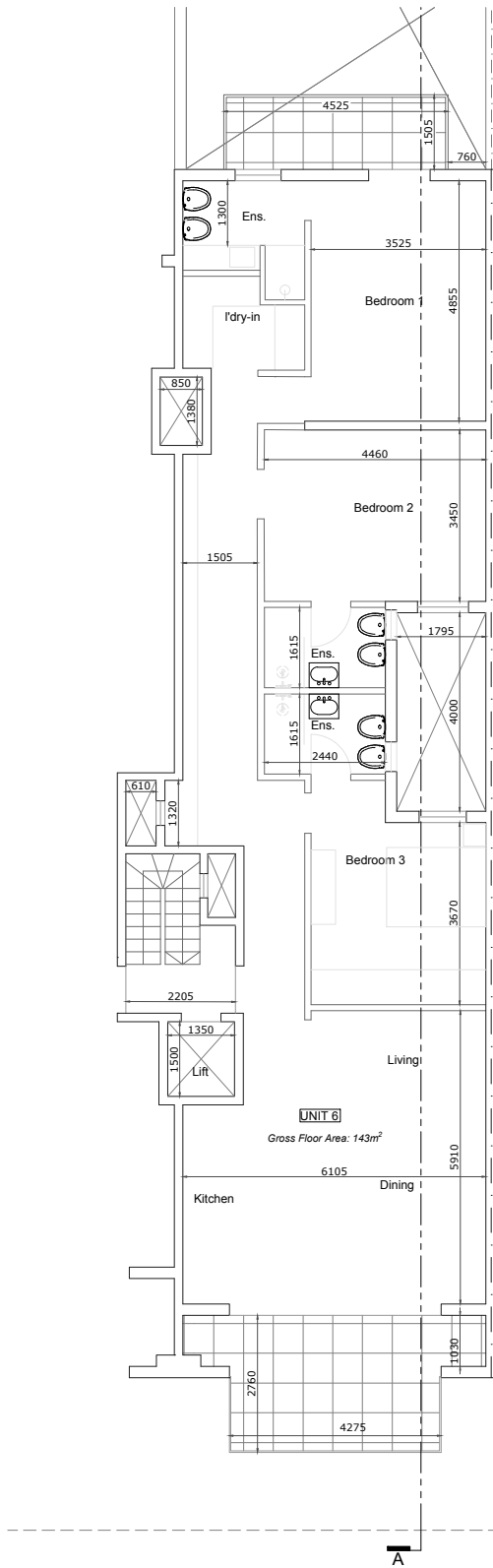
Proposed third floor plan scale 1:100
