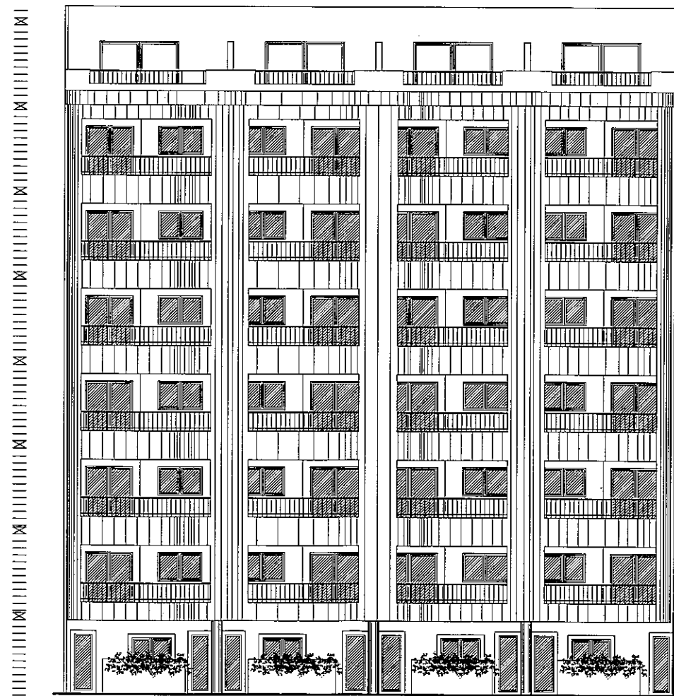
○ Proposed Back Elevation 1
