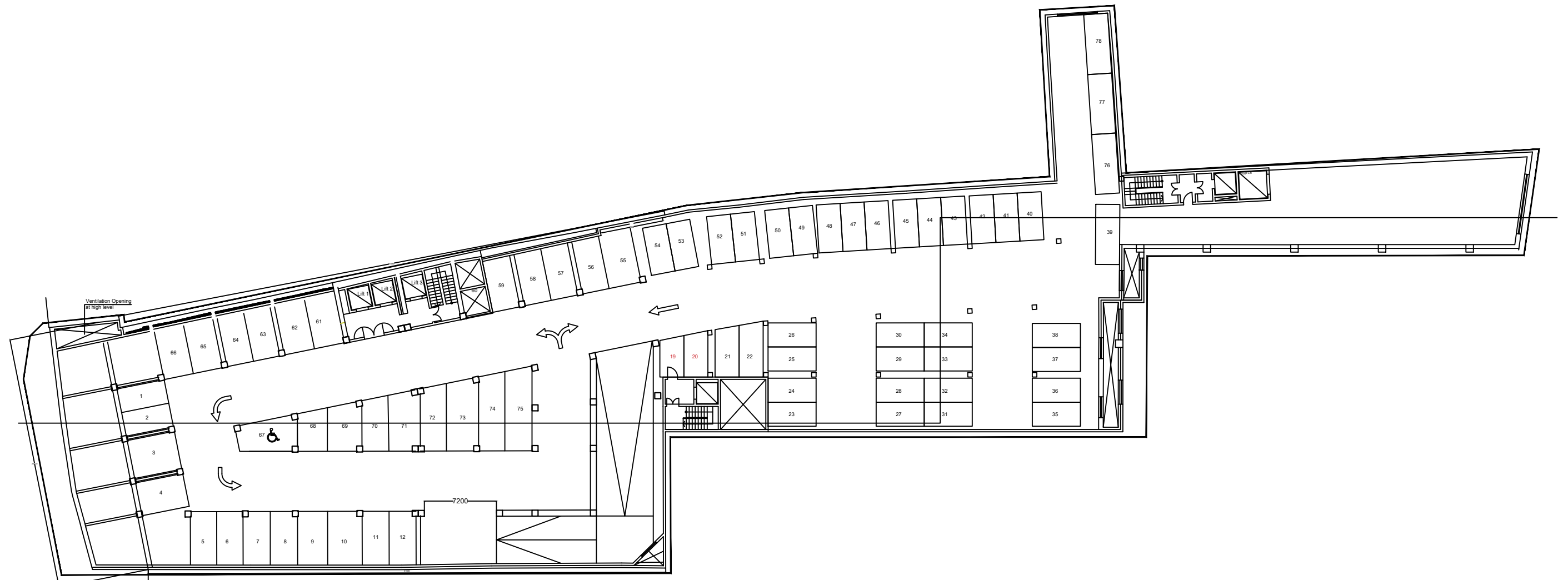
Architectural Layout - Basement level -2 Scale 1:200
