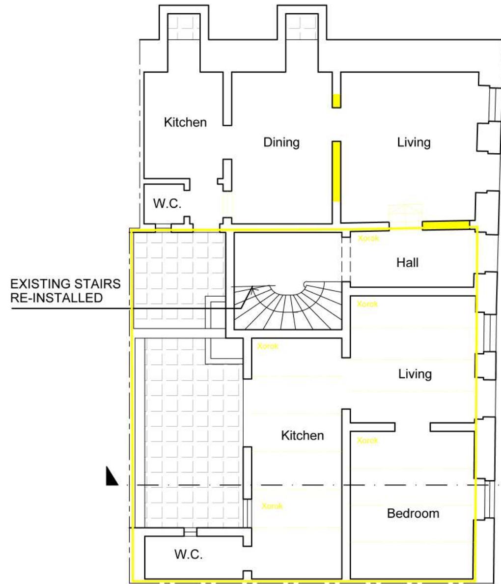
EXISTING UPPER GROUND FLOOR PLAN SCALE 1:100
