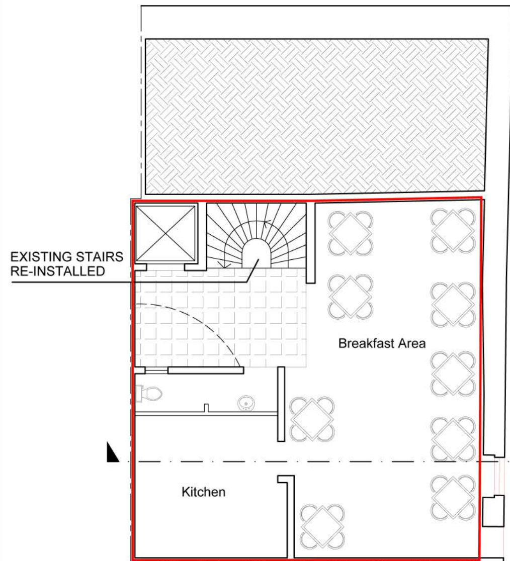
PROPOSED LOWER GROUND FLOOR PLAN SCALE 1:100
