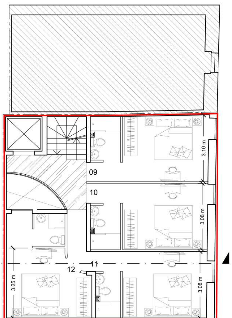
PROPOSED SECOND FLOOR PLAN SCALE 1:100
