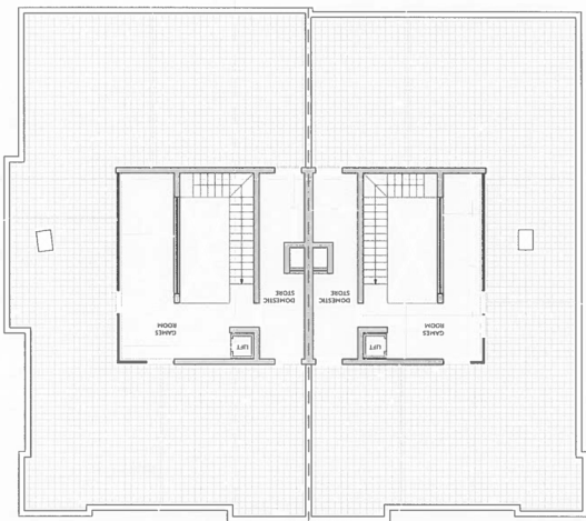
PROPOSED SECOND FLOOR Scale 1:100
