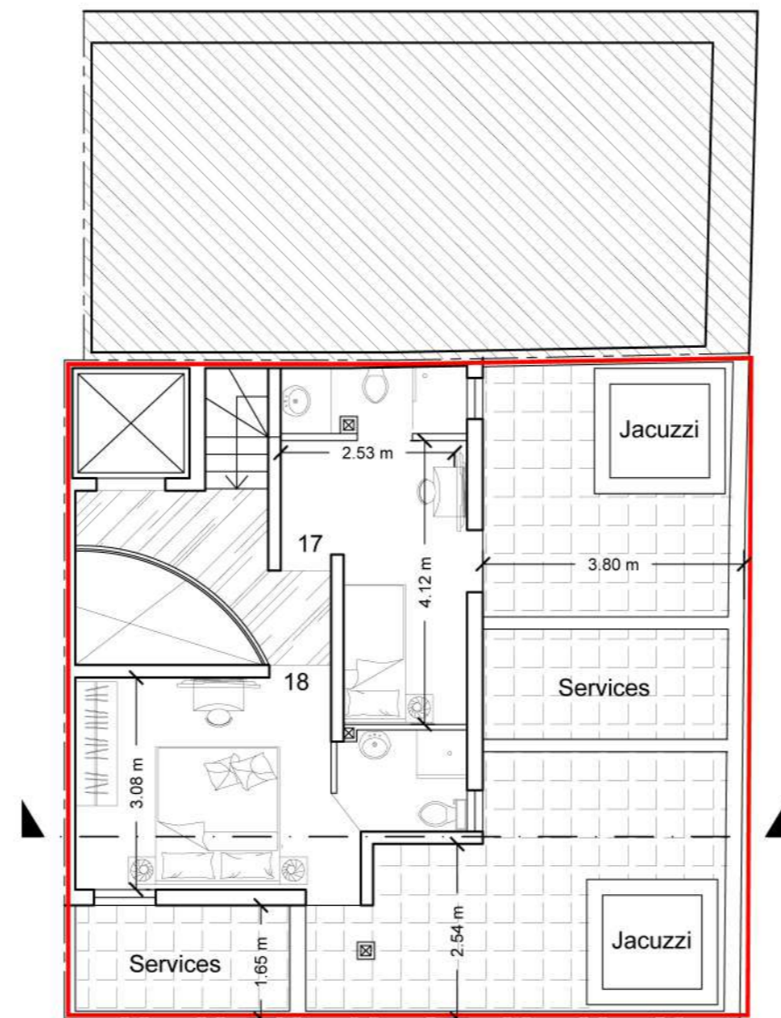
PROPOSED RECEDED FLOOR PLAN SCALE 1:100
