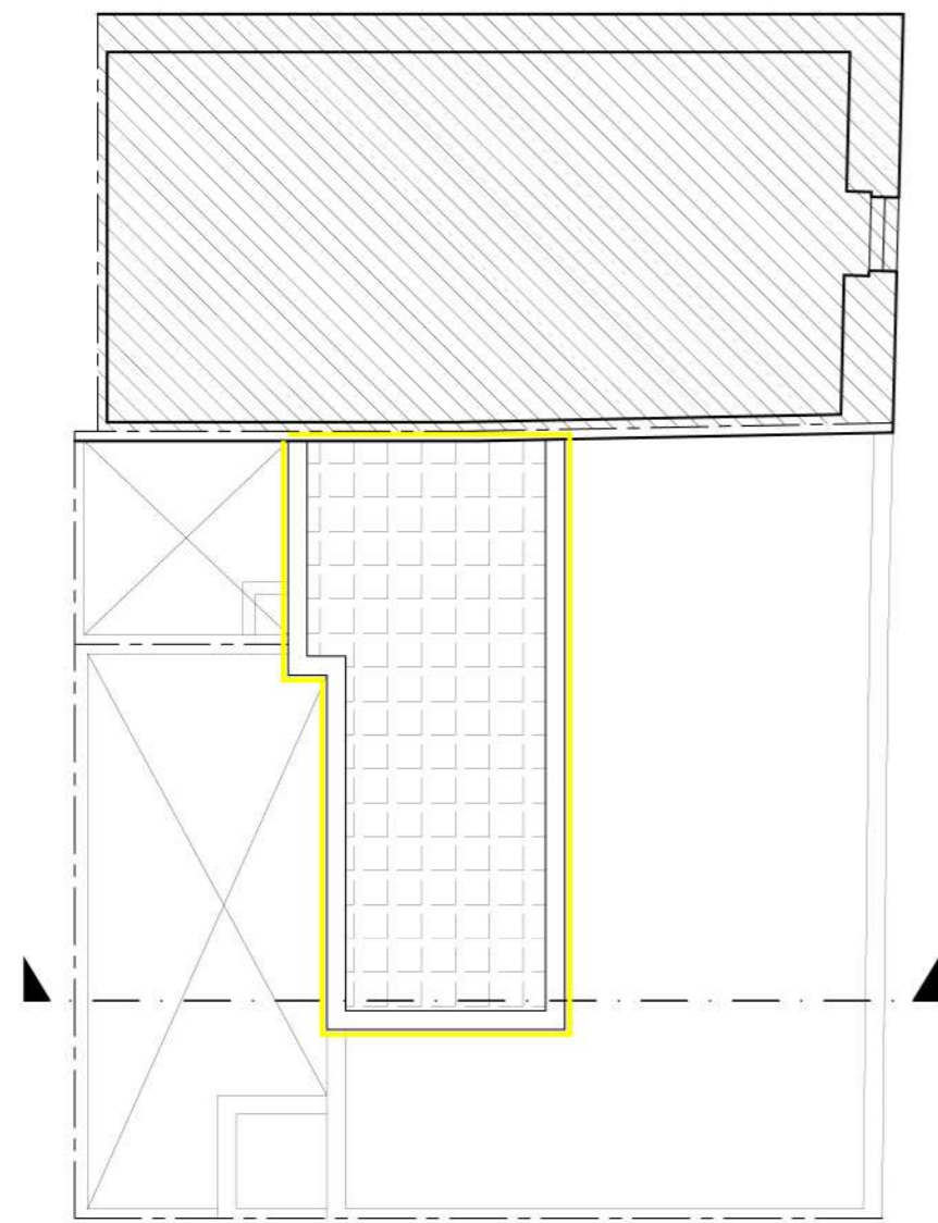
EXISTING THIRD FLOOR PLAN SCALE 1:100
