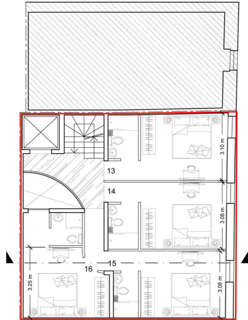
PROPOSED THIRD FLOOR PLAN SCALE 1:100
