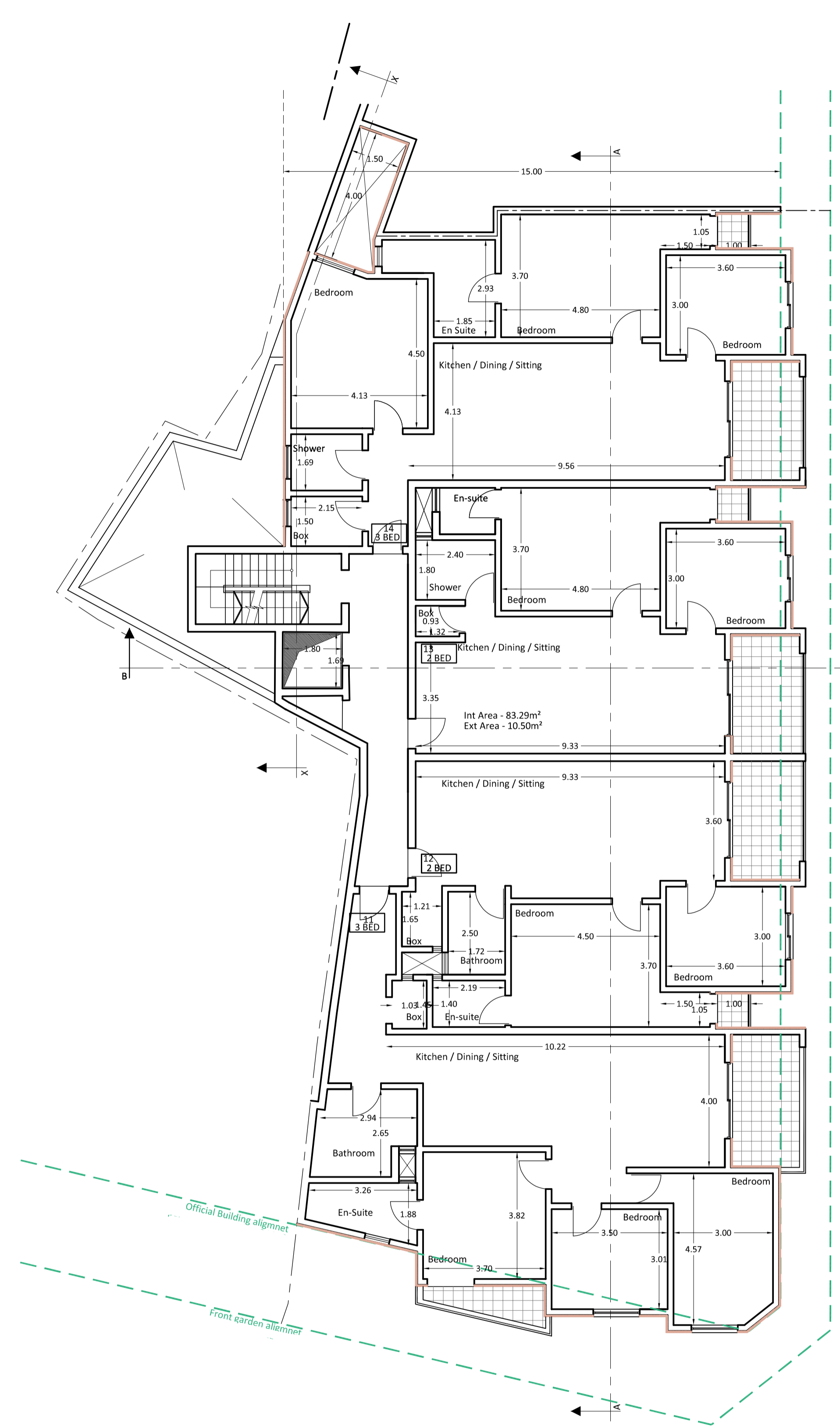
LEVEL 5 SCALE 1:100 PROPOSED
