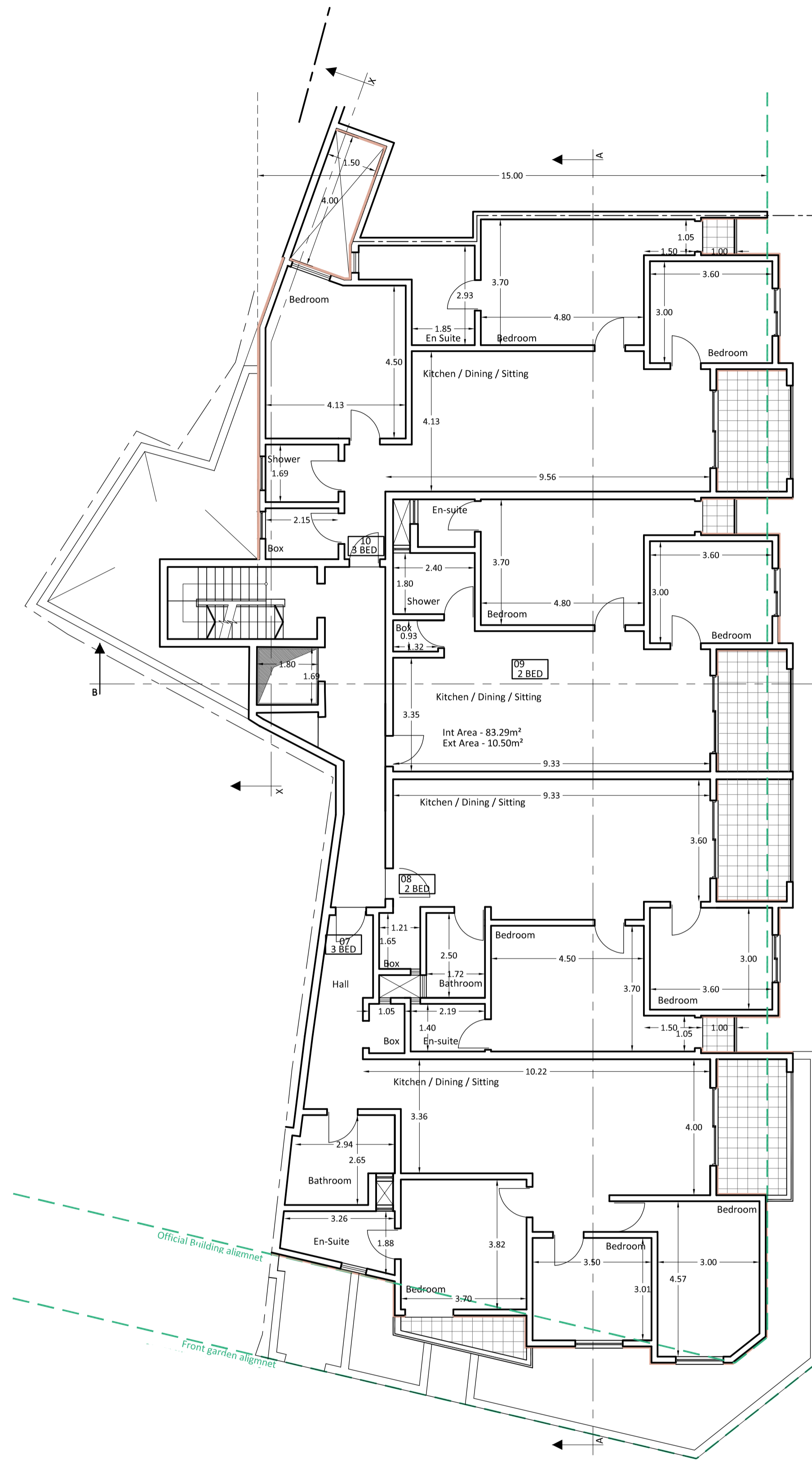
LEVEL 4 SCALE 1:100 PROPOSED
