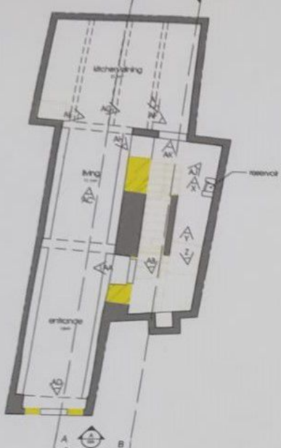
A Existing Ground Floor Plan (Pre 1948) Ref 010 Scale 1:100
