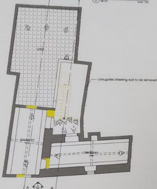
E Proposed First Floor Plan Ref 011 Scale 1:100
