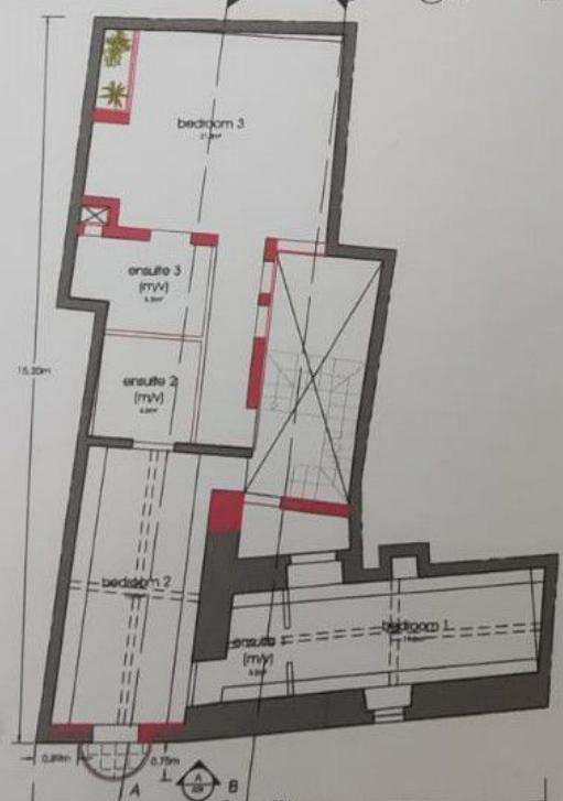
D Proposed Ground Floor Plan Ref 010 Scale 1:100
