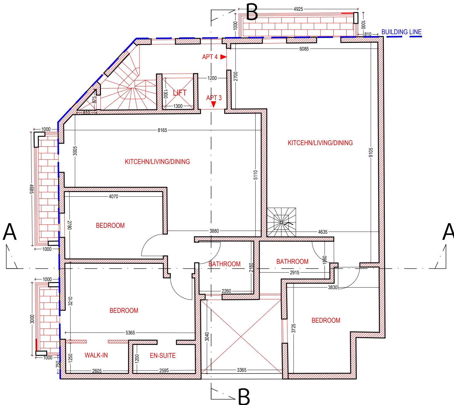
Proposed Second Floor Scale 1:100
