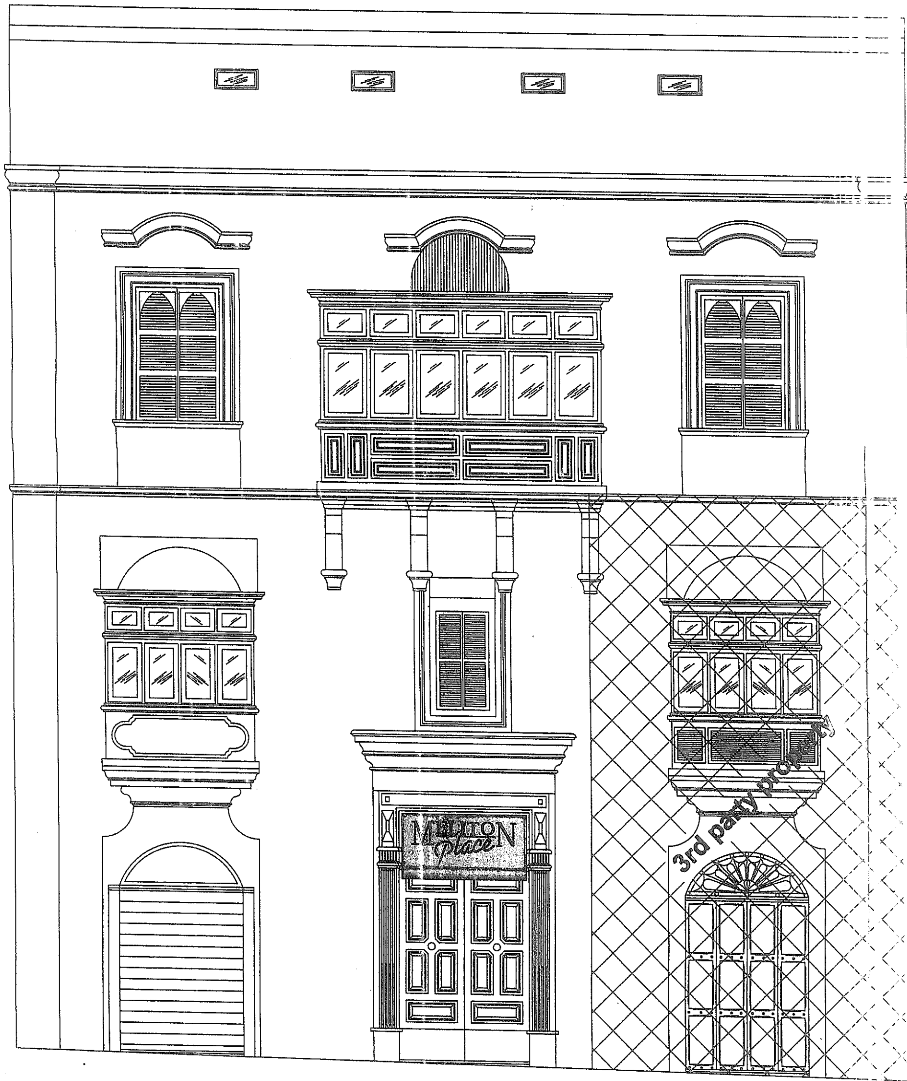
FRONT ELEVATION
