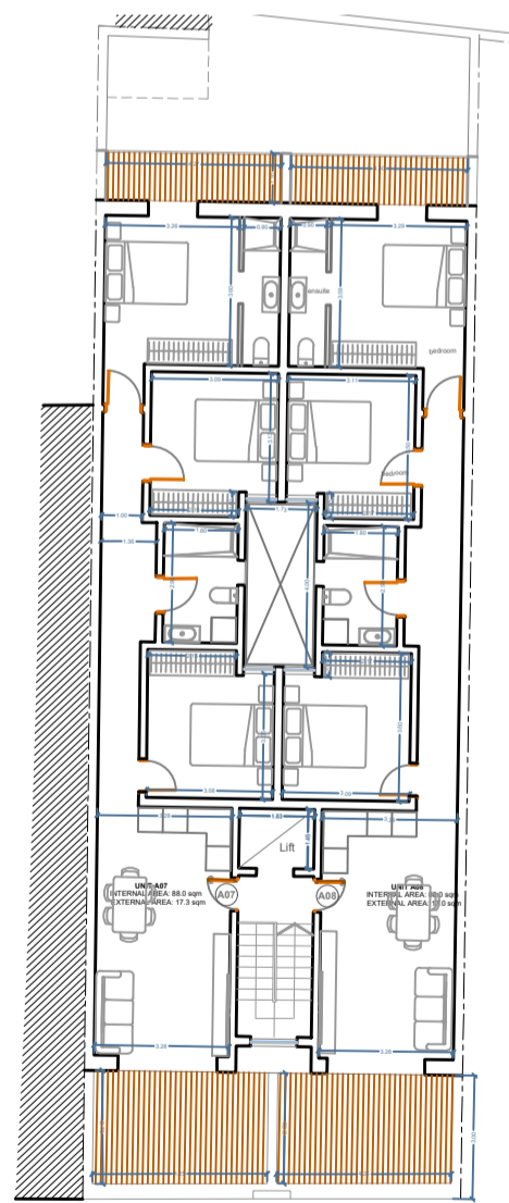
Proposed Floor Level 3 Scale: 1:100 Sheet: 10/3
