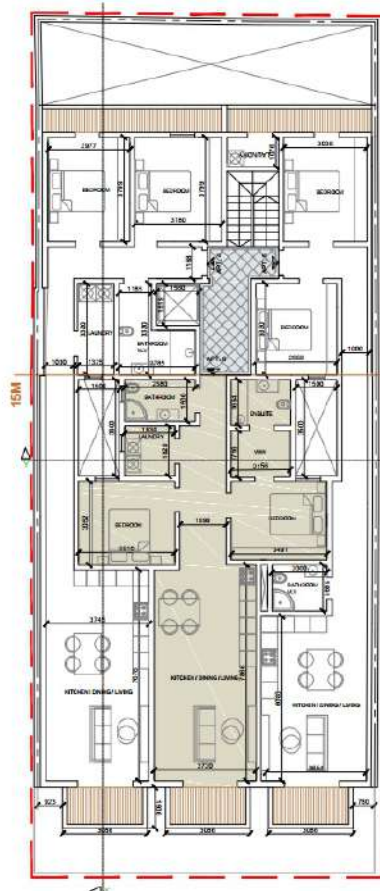
Proposed Second Floor Scale 1:100
