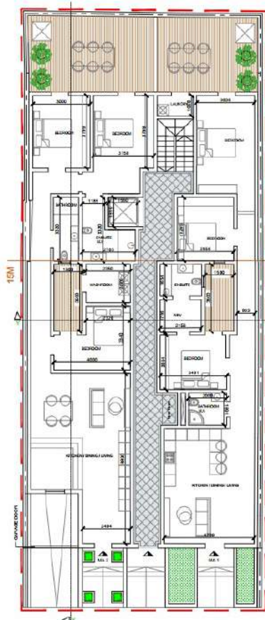
Proposed Elevated Ground Floor Scale 1:100
