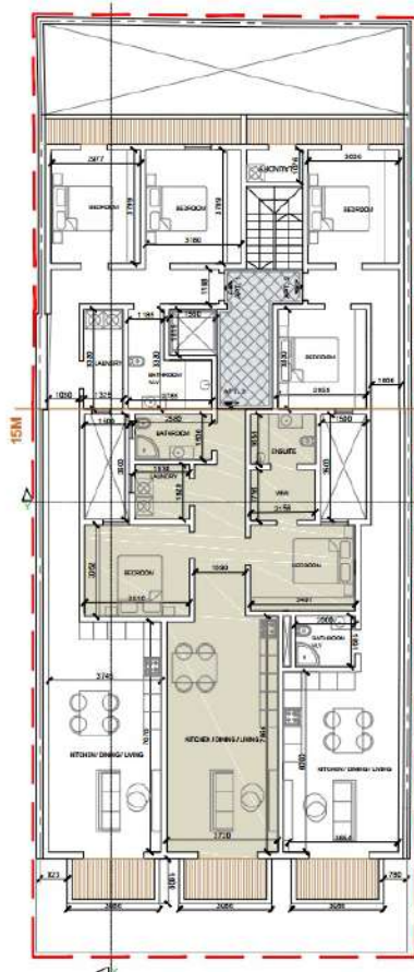
Proposed First Floor Scale 1:100
