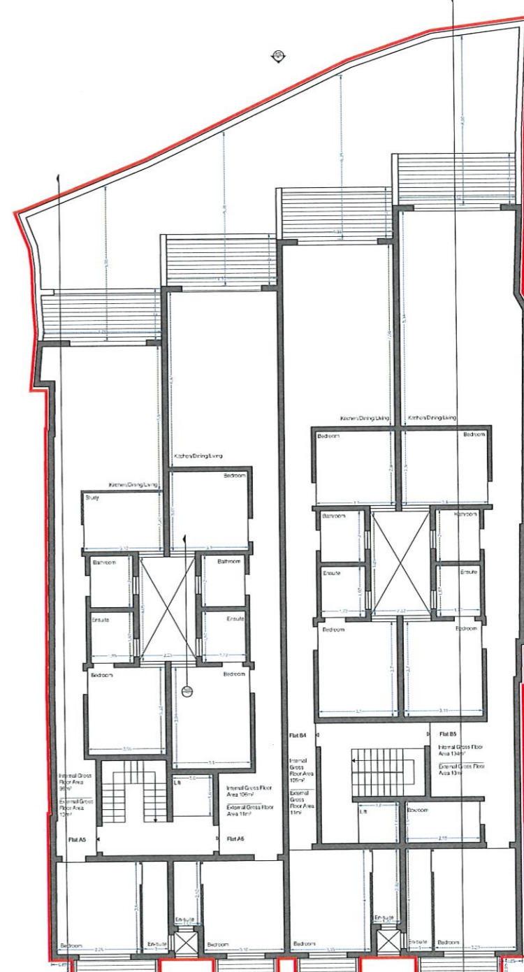
Proposed Second Floor Plan Scale 1:100
