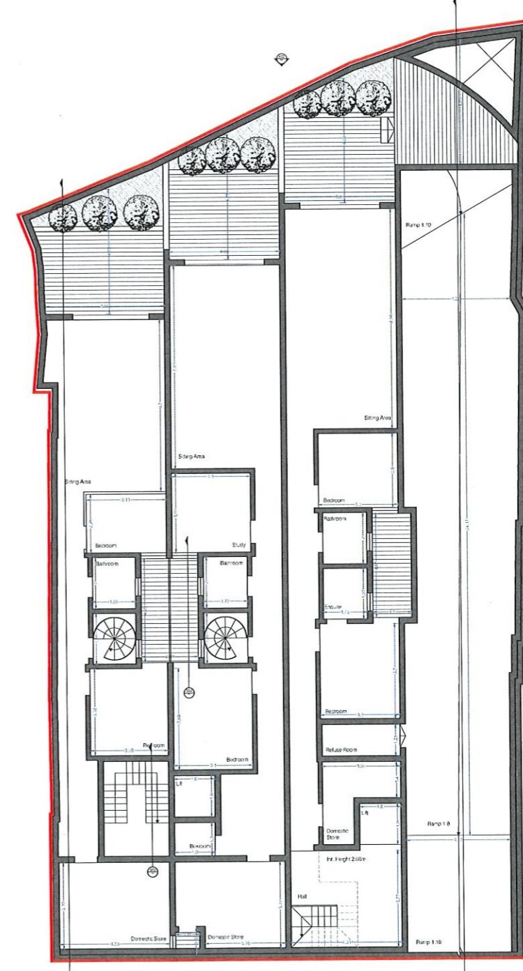
Proposed Basement -1 Floor Plan Scale 1:100
