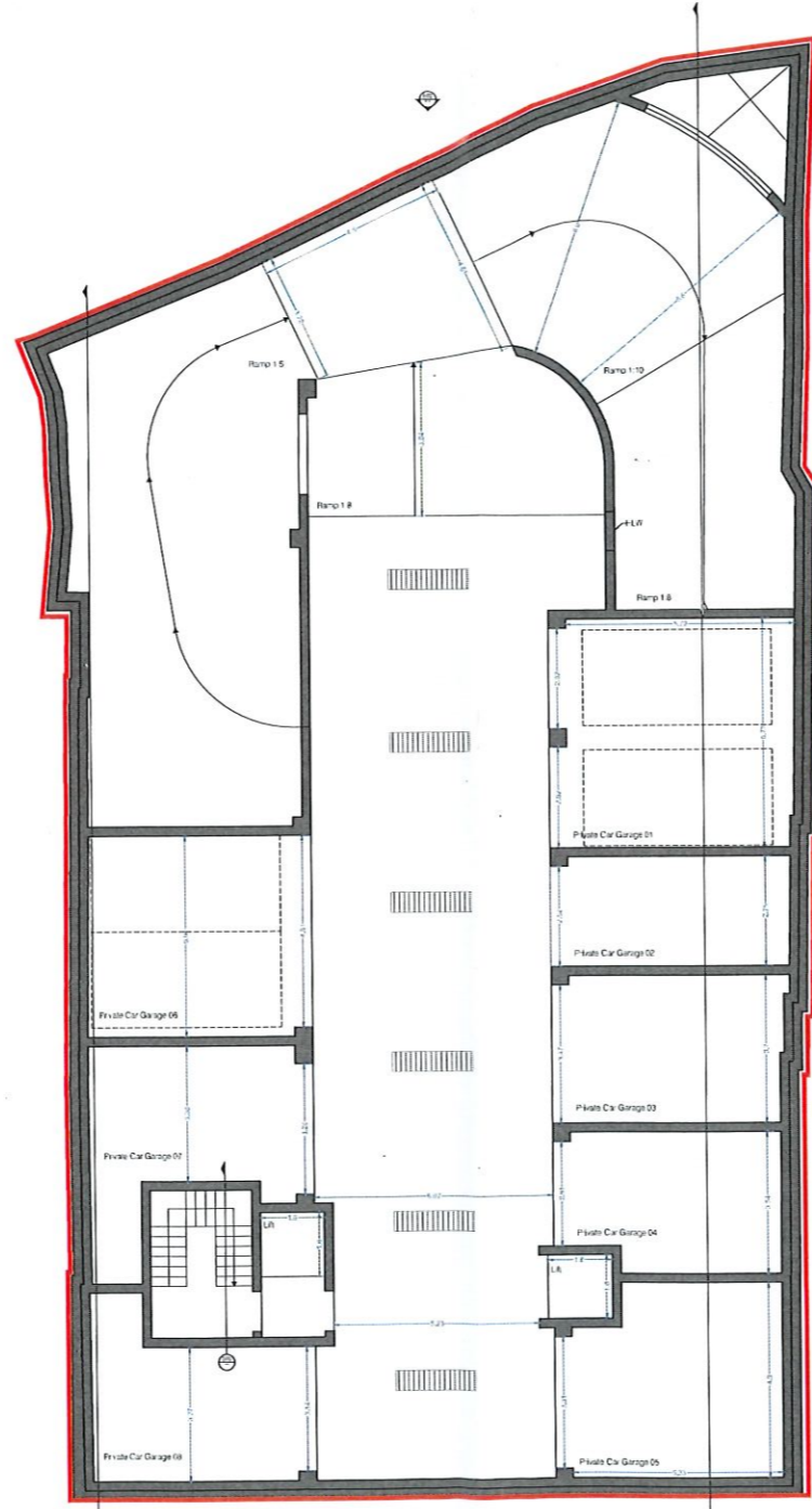
Proposed Basement -2 Floor Plan Scale 1:100
