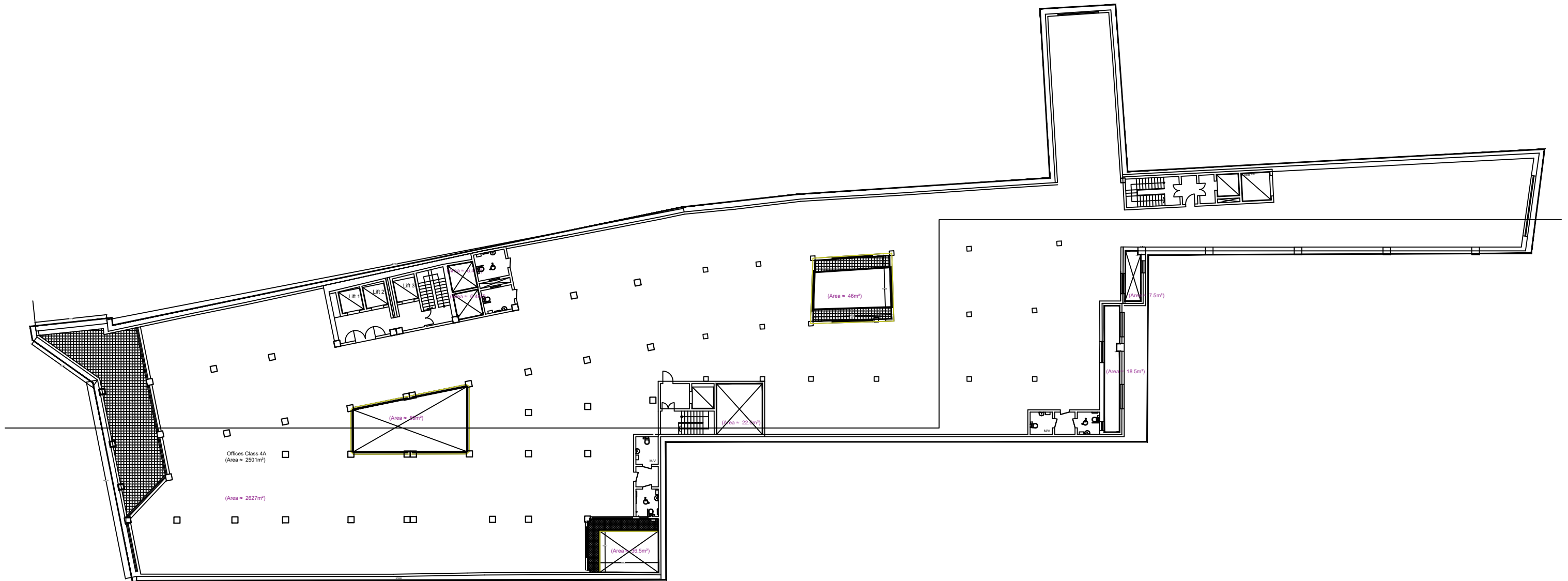
Architectural Layout - 1st floor level Scale 1:200
