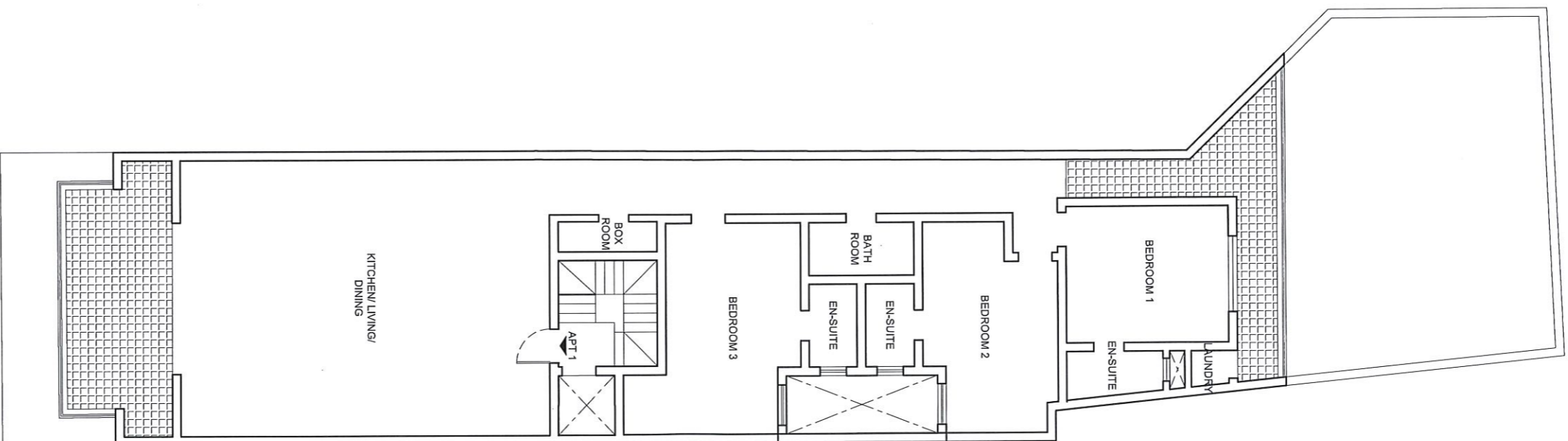
PROPOSED FIRST FLOOR LAYOUT Scale 1:100
