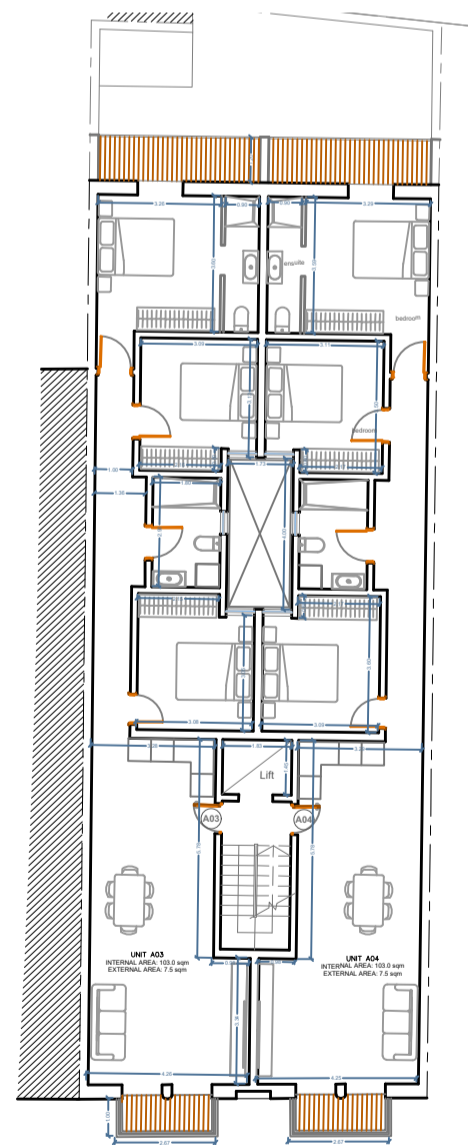
Proposed Floor Scale 1:100 (over copy)
