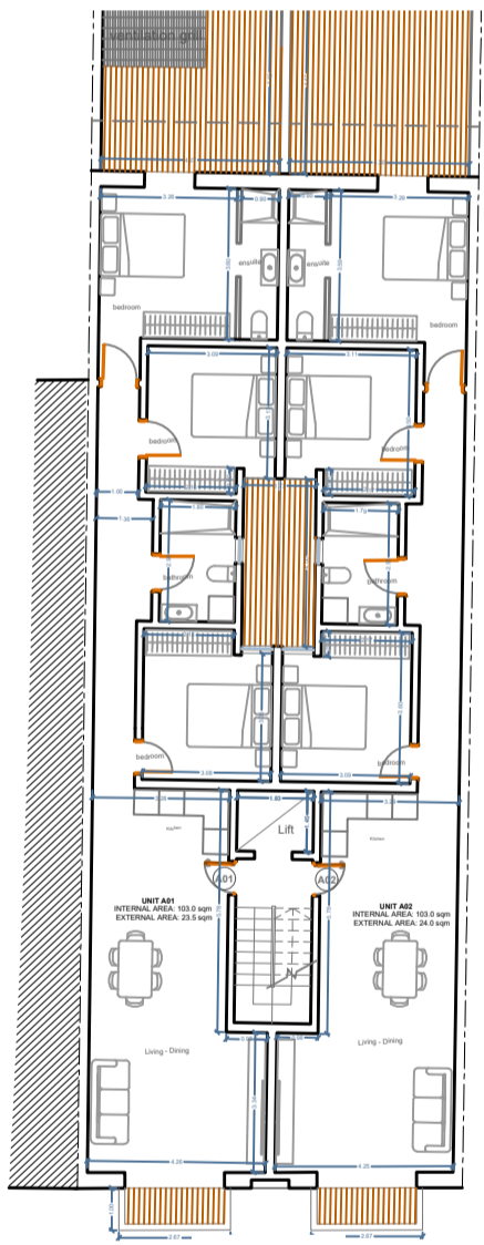
Proposed Floor L Scale 1:100 (over copy)
