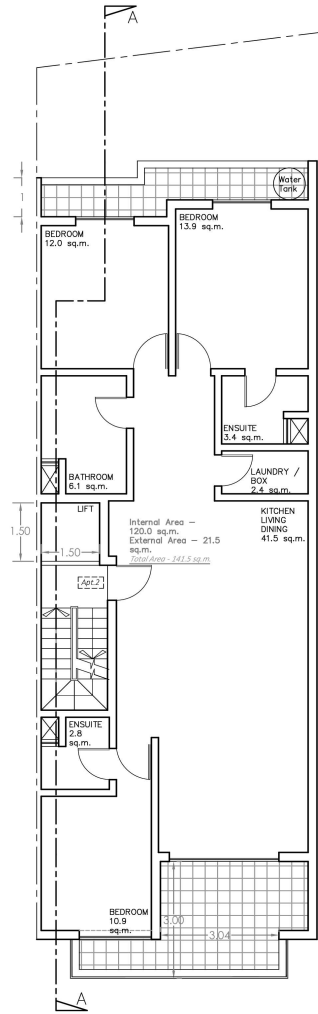
PROPOSED FIRST FLOOR
