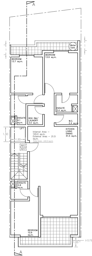
PROPOSED SECOND & THIRD FLOOR
