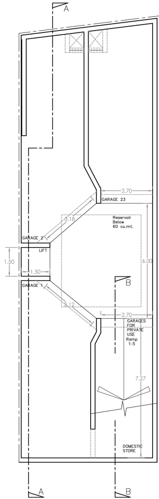
PROPOSED BASEMENT LEVEL
