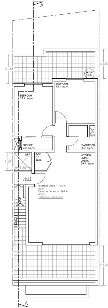
PROPOSED PENTHOUSE LEVEL
