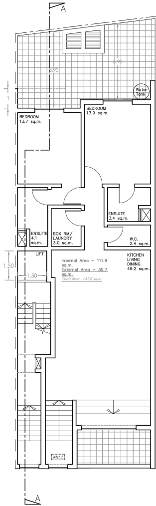
PROPOSED GROUND FLOOR
