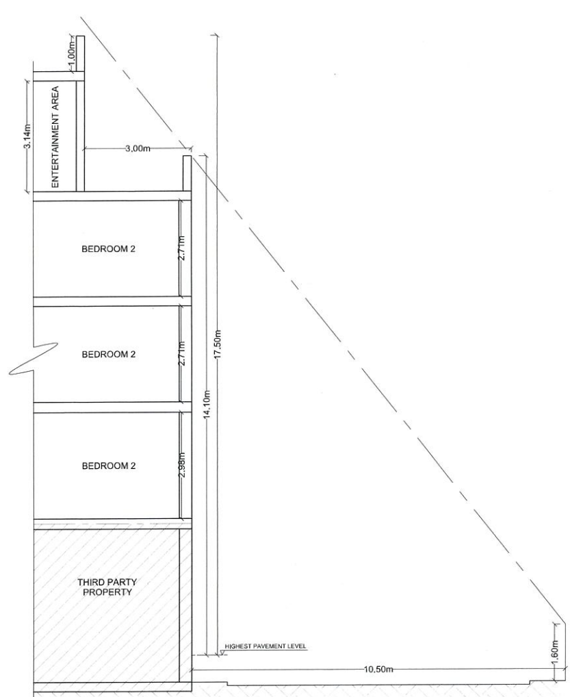
PROPOSED PART SECTION D-D SCALE 1:50
