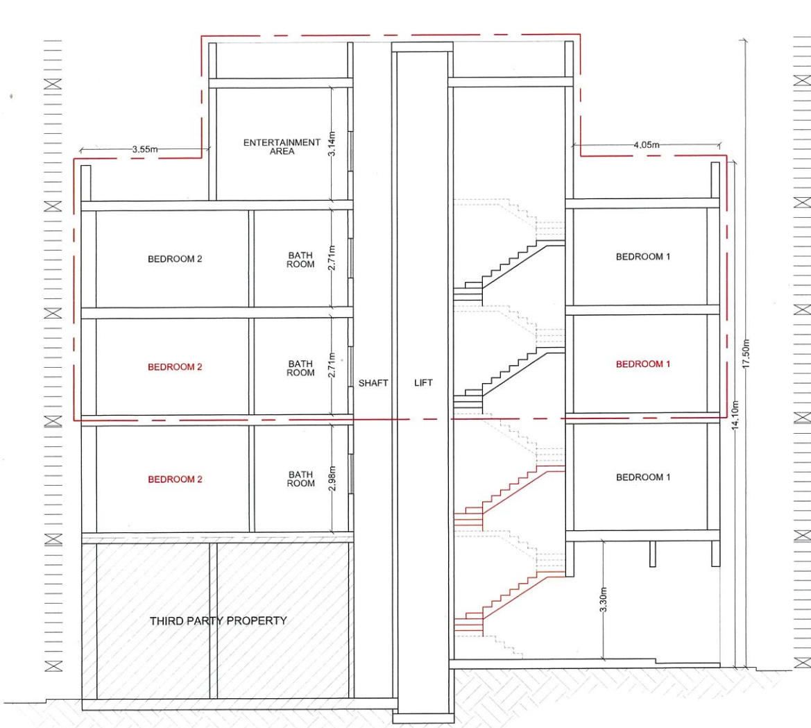
PROPOSED SECTION A-A SCALE 1:50
