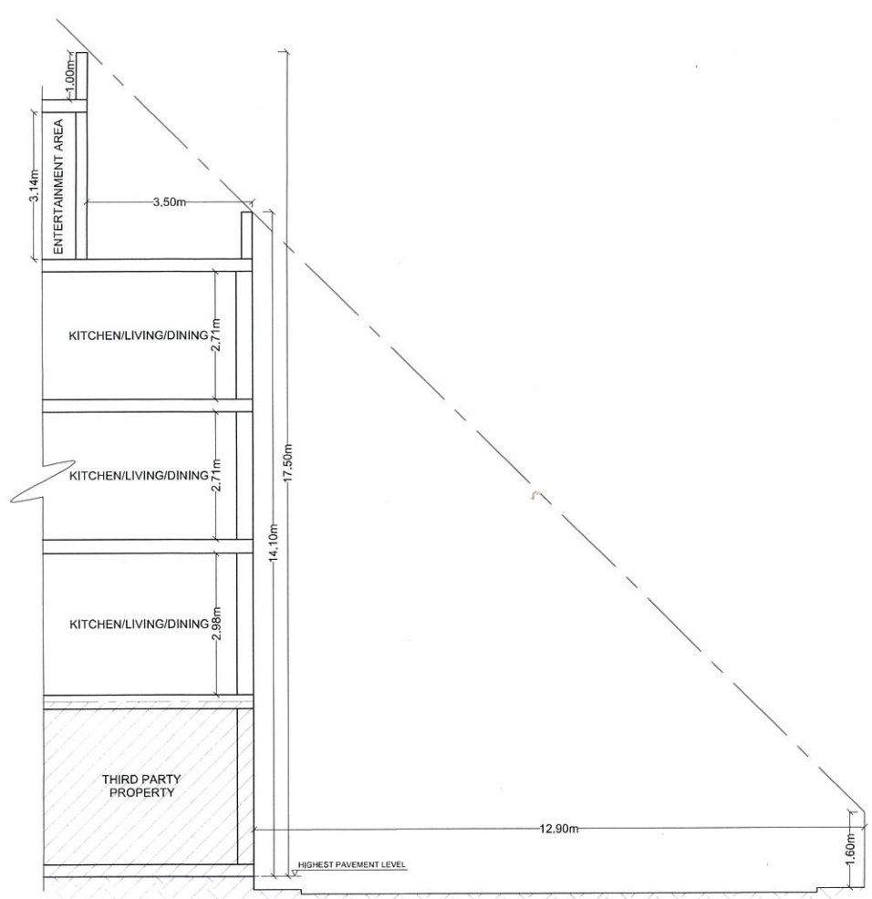
PROPOSED PART SECTION C-C SCALE 1:50
