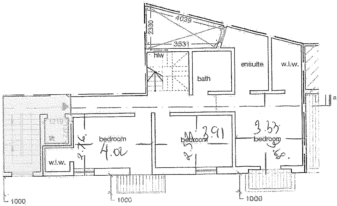
proposed second floor level
