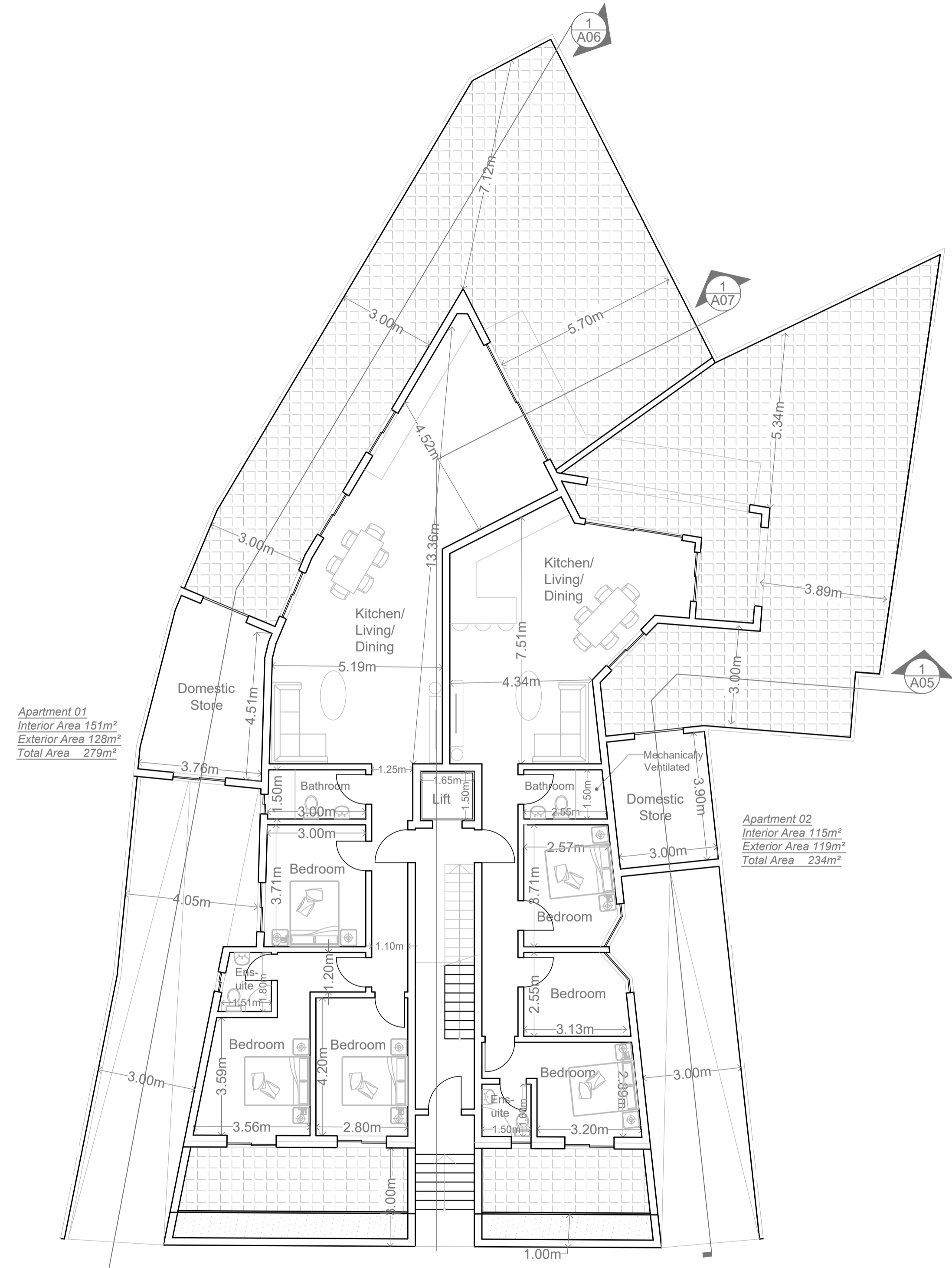
01 Proposed Ground Floor A02 Scale 1:100 on A1
