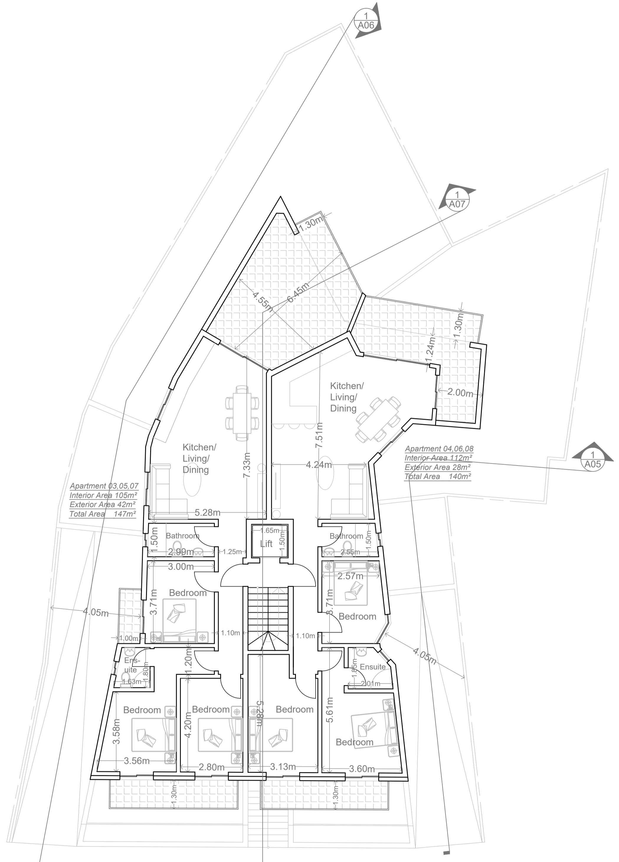
02 Proposed 1st, 2nd & 3rd Floor A02 Scale 1:100 on A1
