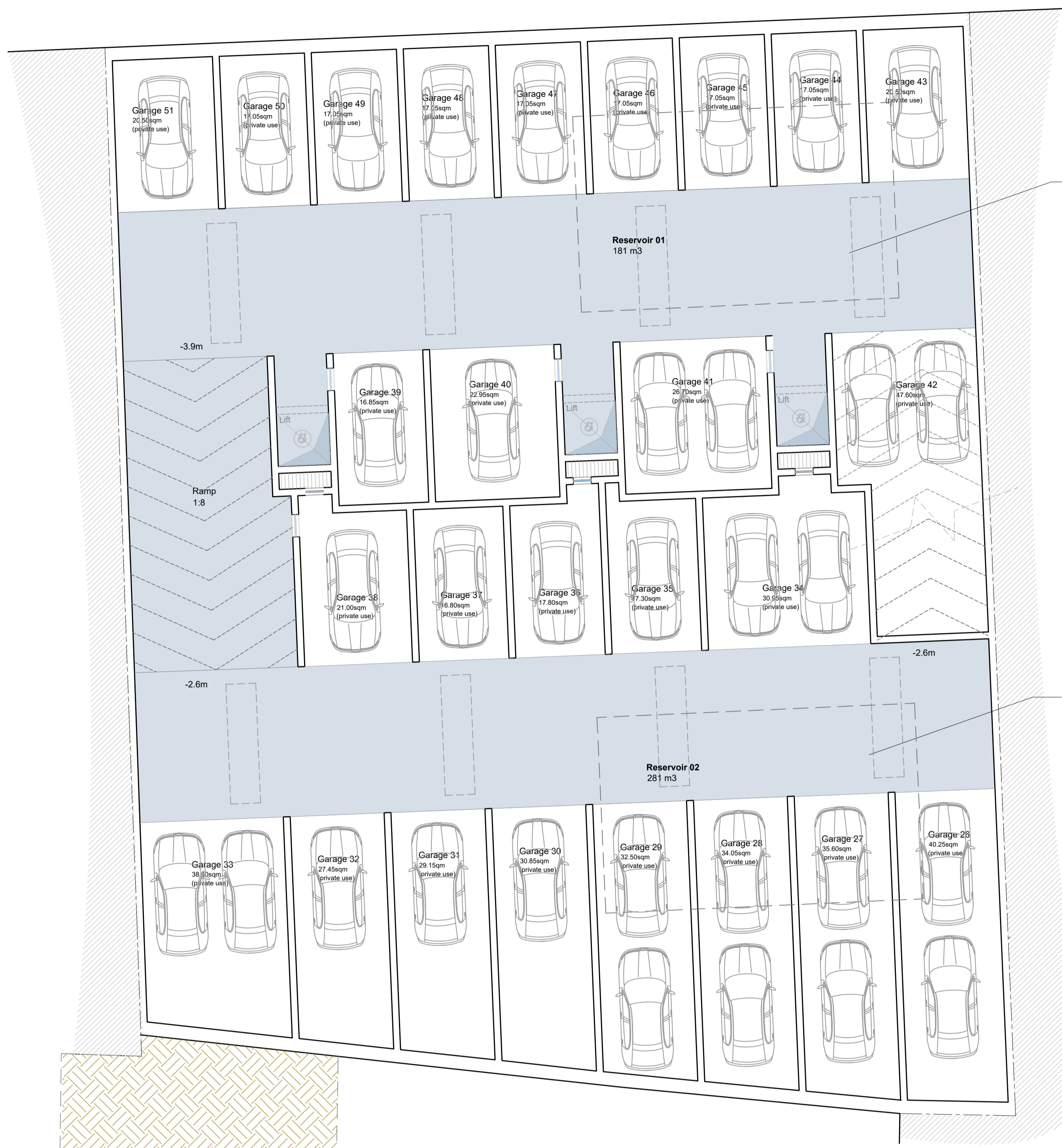
Proposed Floor Level -2 Scale: 1:100 Sheet copy
