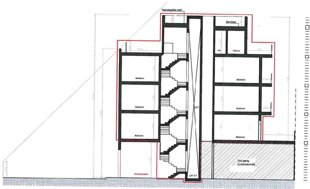
Proposed Section BB Scale 1:100
