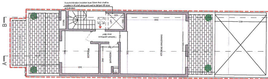
PROPOSED RECEDED FLOOR Scale 1:100
