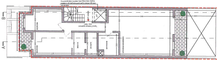
PROPOSED TYPICAL FLOOR Scale 1:100
