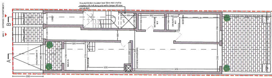
PROPOSED GROUND FLOOR Scale 1:100
