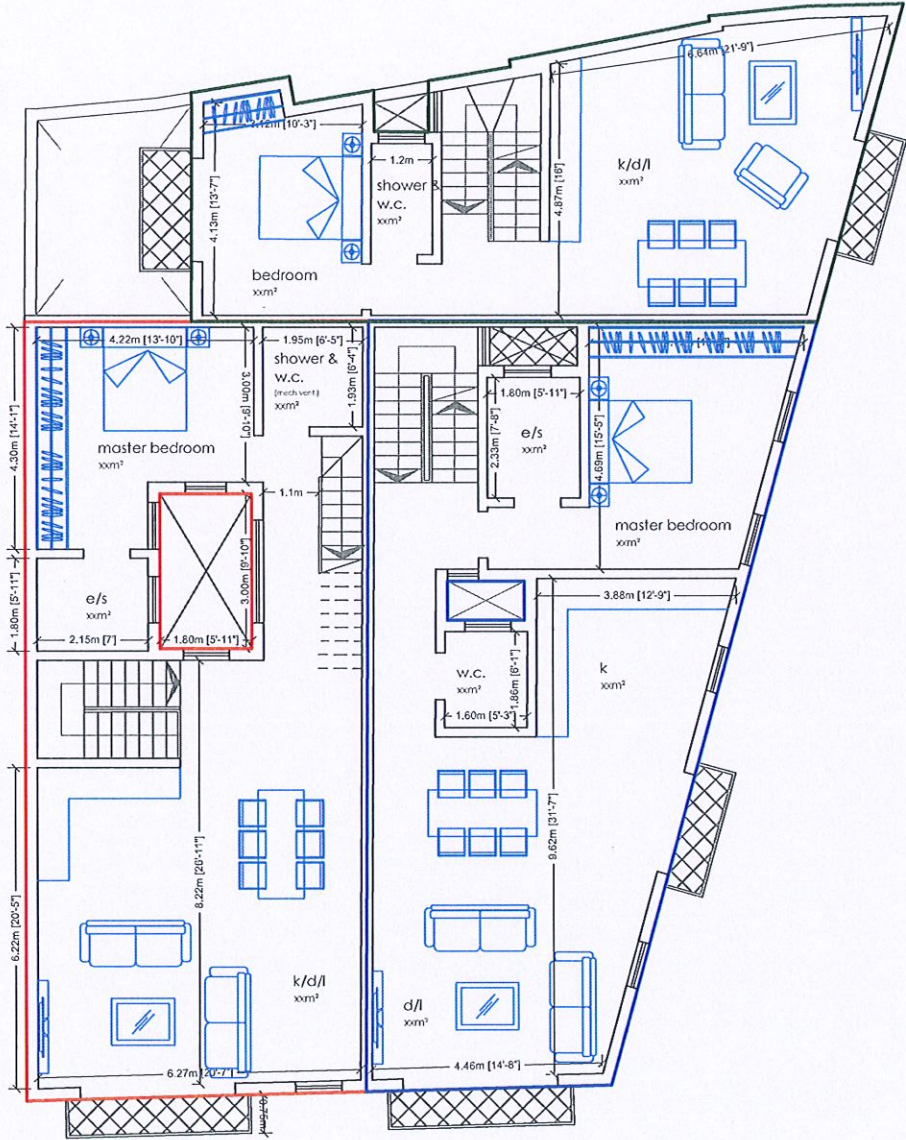
Proposed First Floor Level Plan Scale 1:100
