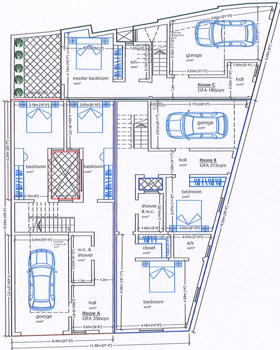
Proposed Ground Floor Level Plan Scale 1:100
