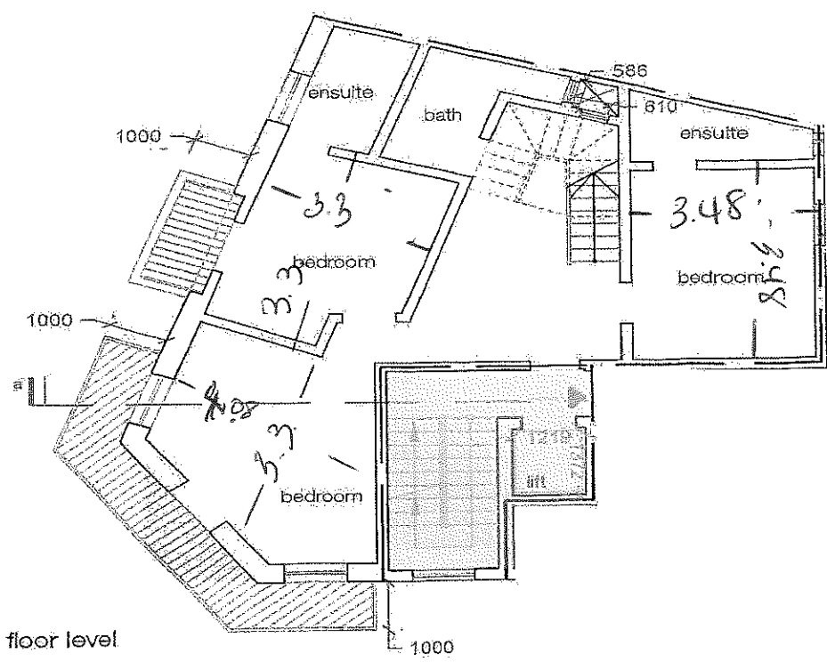
proposed recessed floor level
