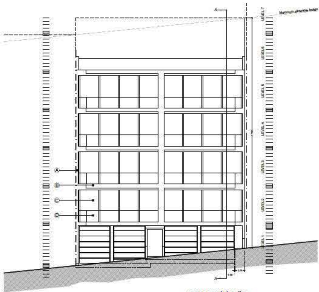
As Approved Elevation Scale 1:100
