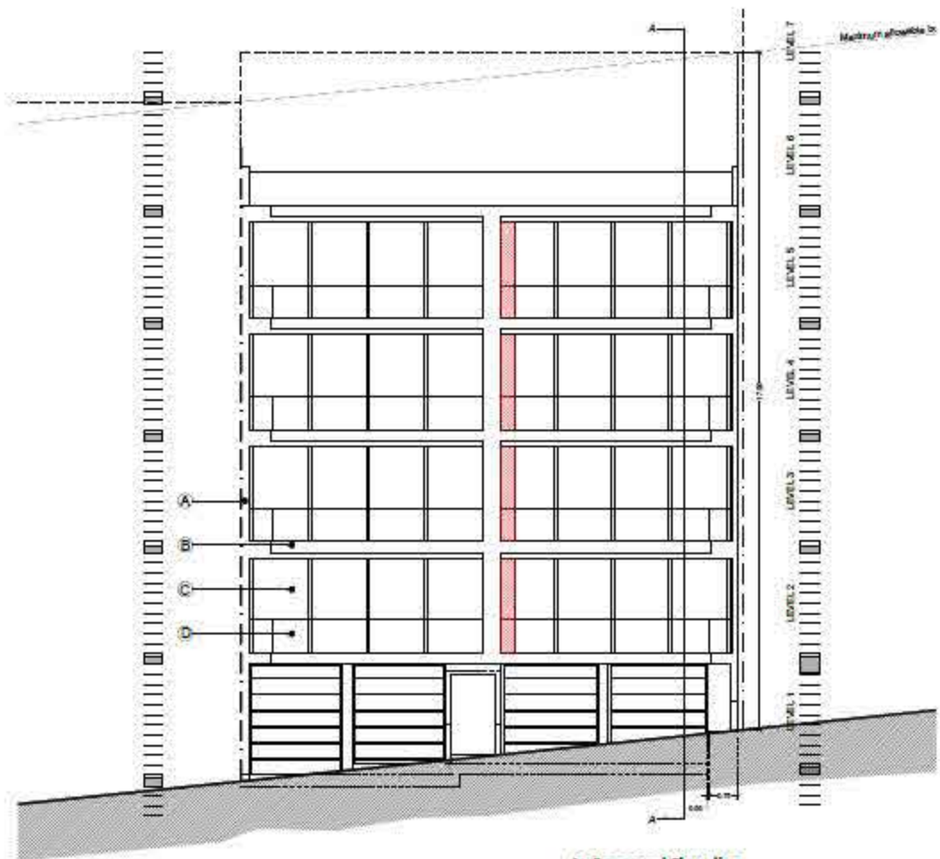
As Proposed Elevation Scale 1:100
