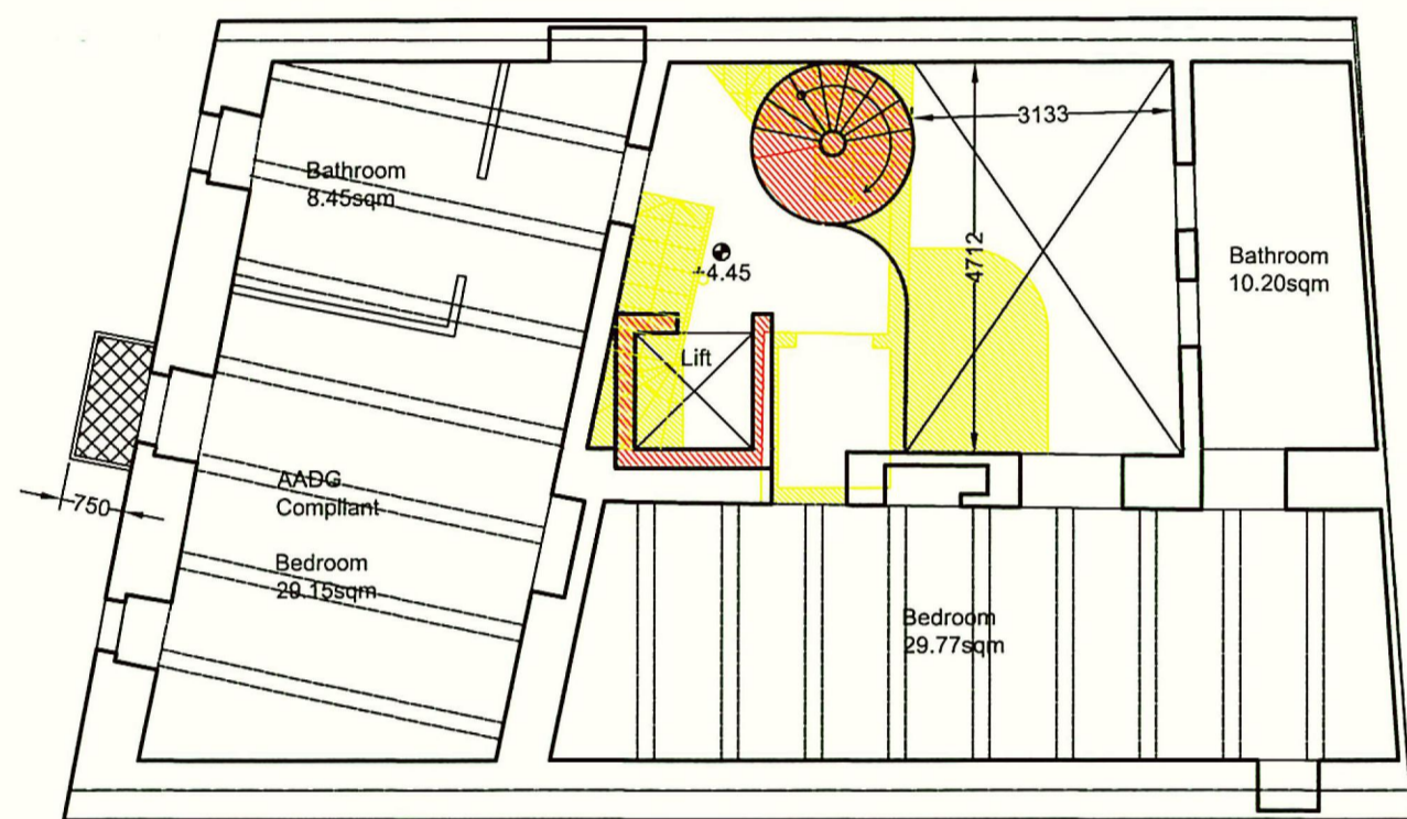
PROPOSED FIRST LEVEL Scale 1:100
