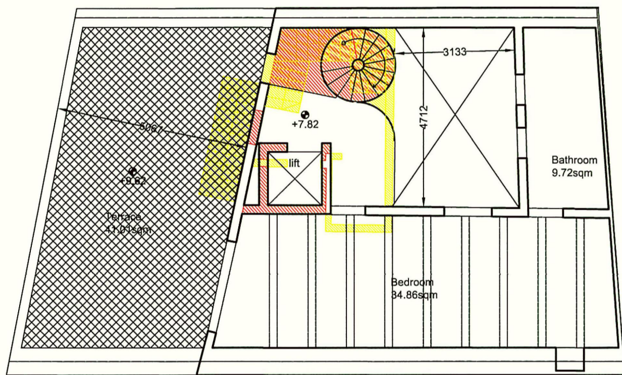
PROPOSED SECOND LEVEL Scale 1:100
