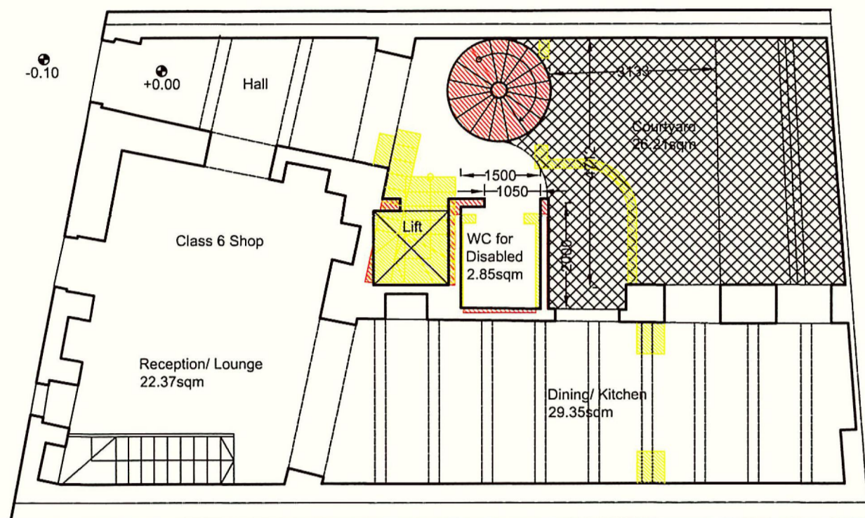
PROPOSED GROUND LEVEL Scale 1:100
