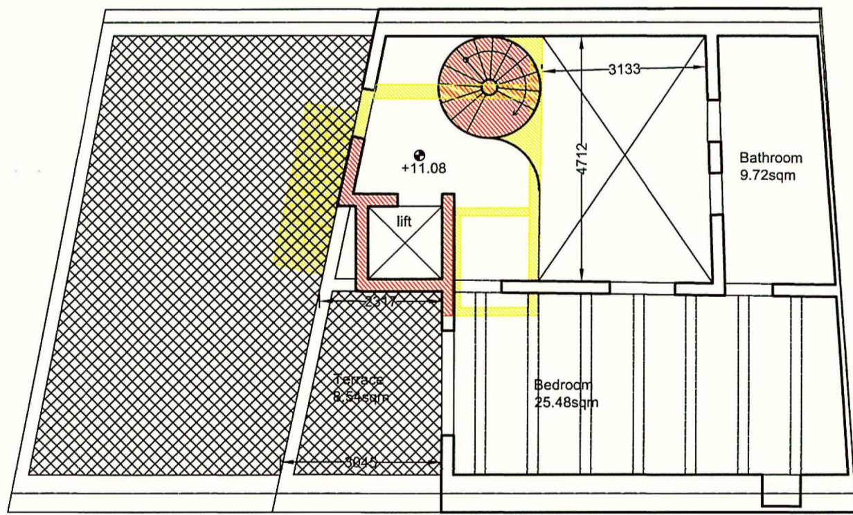
PROPOSED RECEDED THIRD LEVEL Scale 1:100
