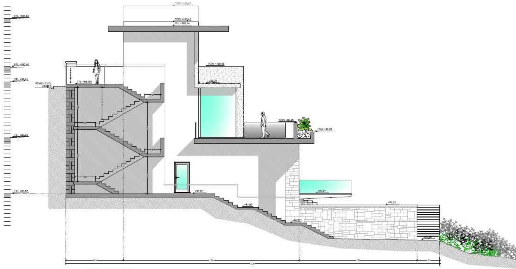
NORTH WEST ELEVATION SCALE 1/8"
