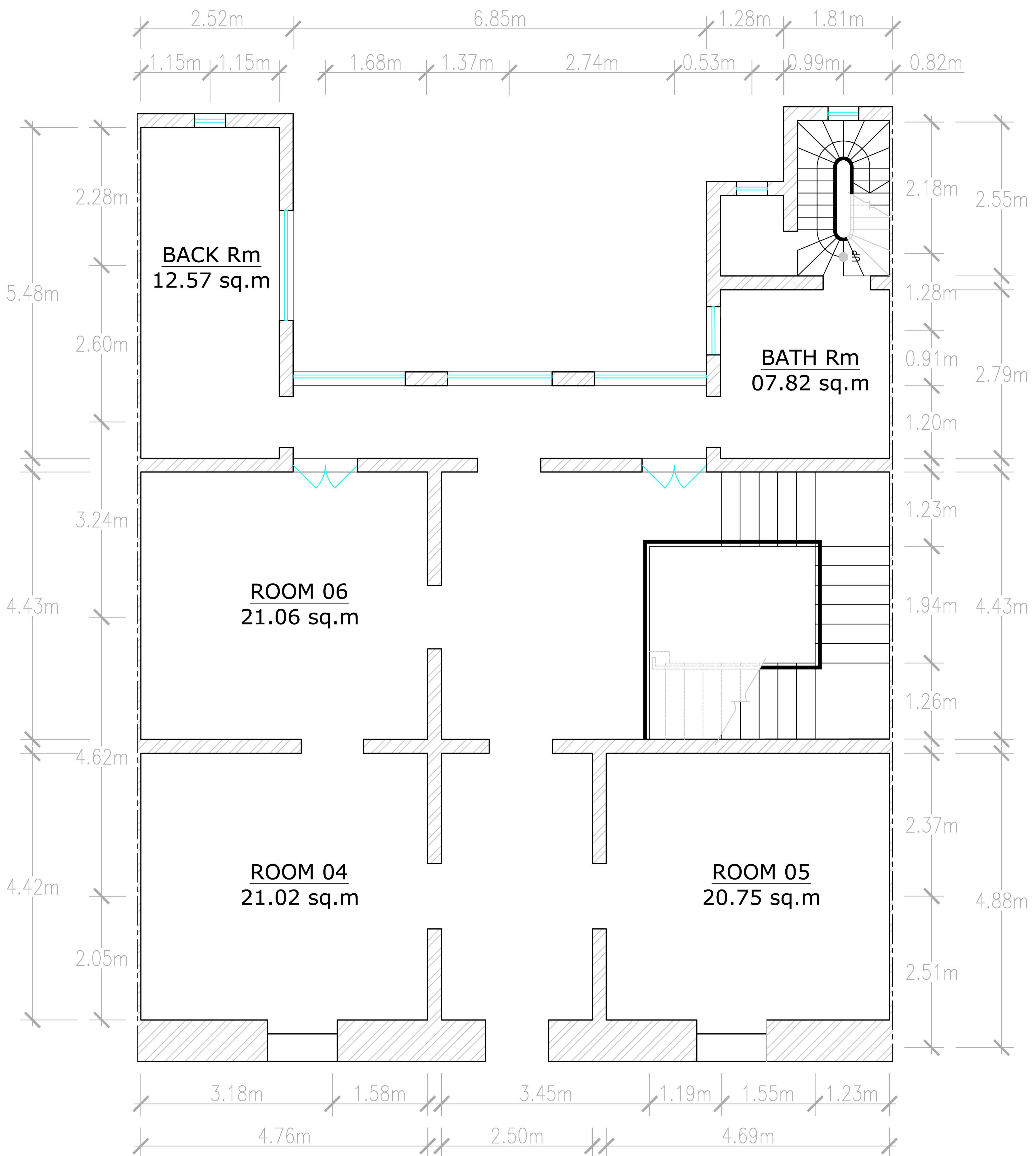
FIRST FLOOR PLAN
