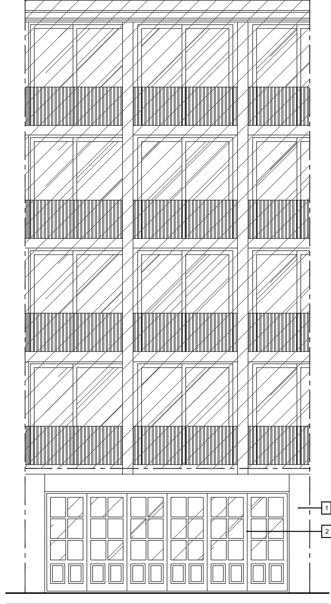
EXISTING ELEVATION Scale 1:100
