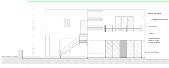
① Approved Elevation Scale 1:50
