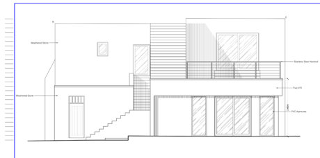
② Existing Elevation BC Scale 1:50
