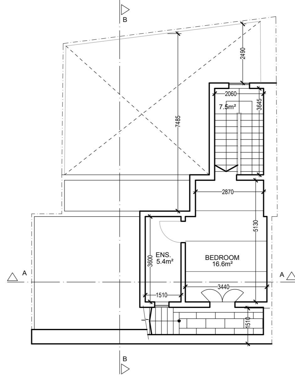
EXISTING SECOND FLOOR PLAN Scale 1:100
