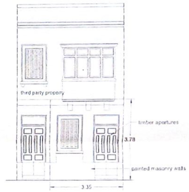
EXISTING ELEVATION
