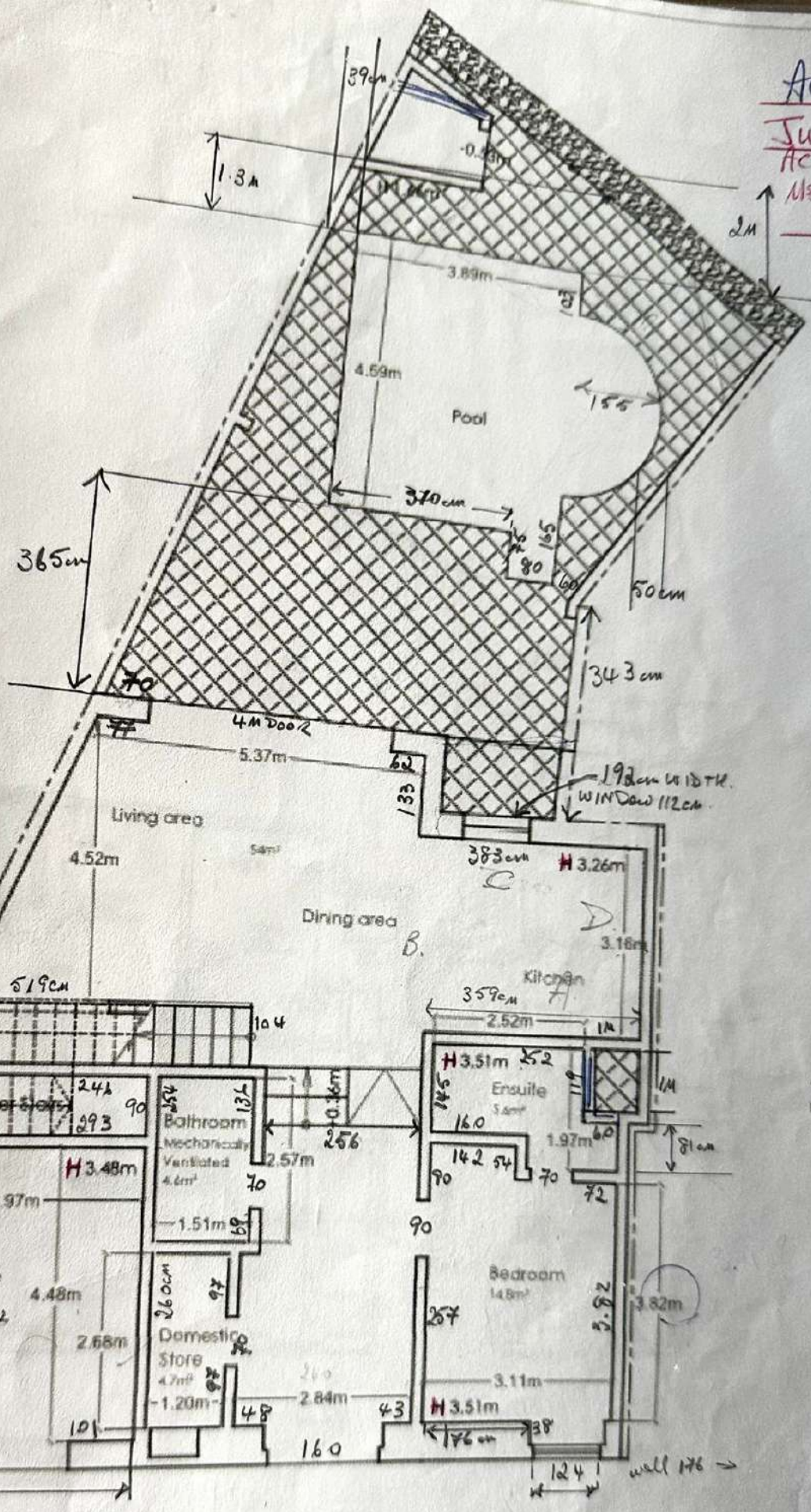
Proposed Ground Floor Level Plan clean copy
