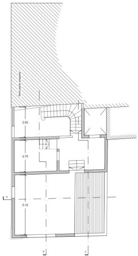
second floor as approved in PA - scale 1:100
