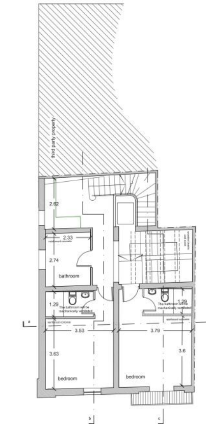
first floor - as proposed - scale 1:100
