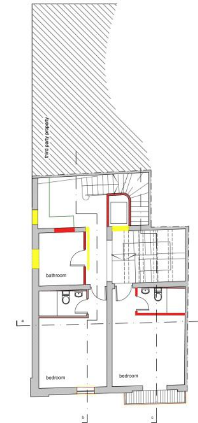
first floor - as existing/ proposed - scale 1:100
