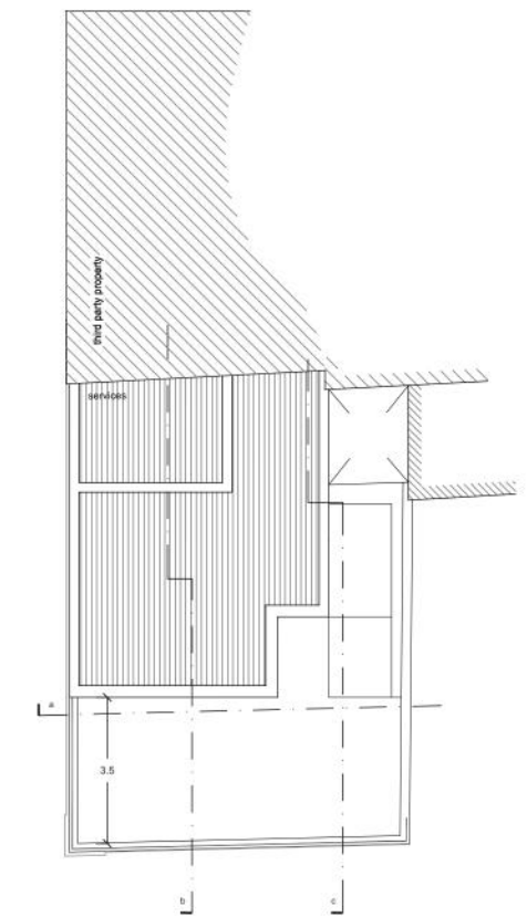
roof plan - as proposed - scale 1:100
