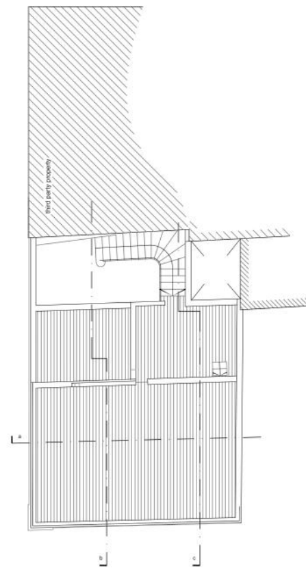
second floor - as existing - scale 1:100
