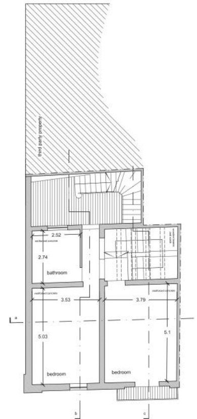
first floor - as existing - scale 1:100
