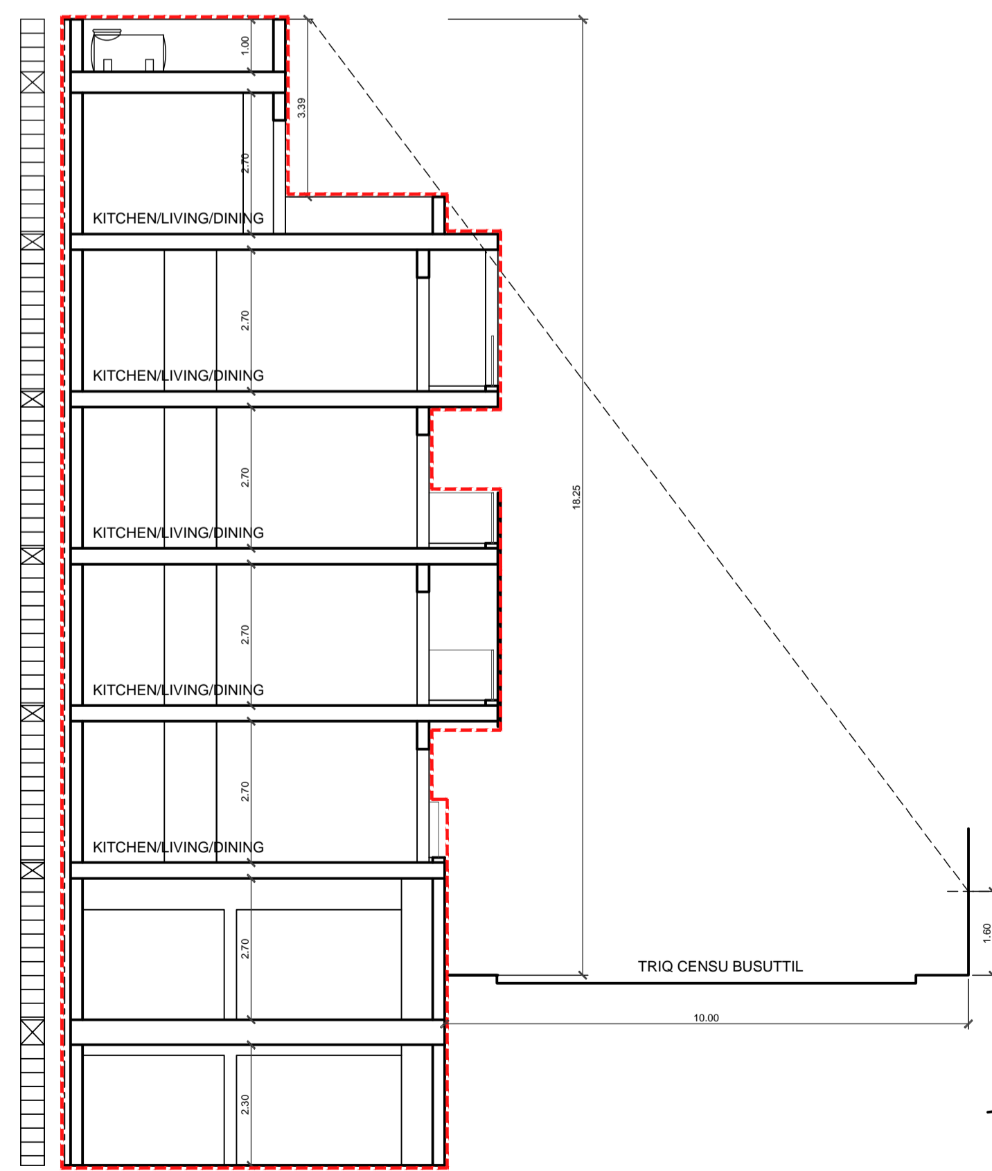
3 Proposed Section X-X 1:100
