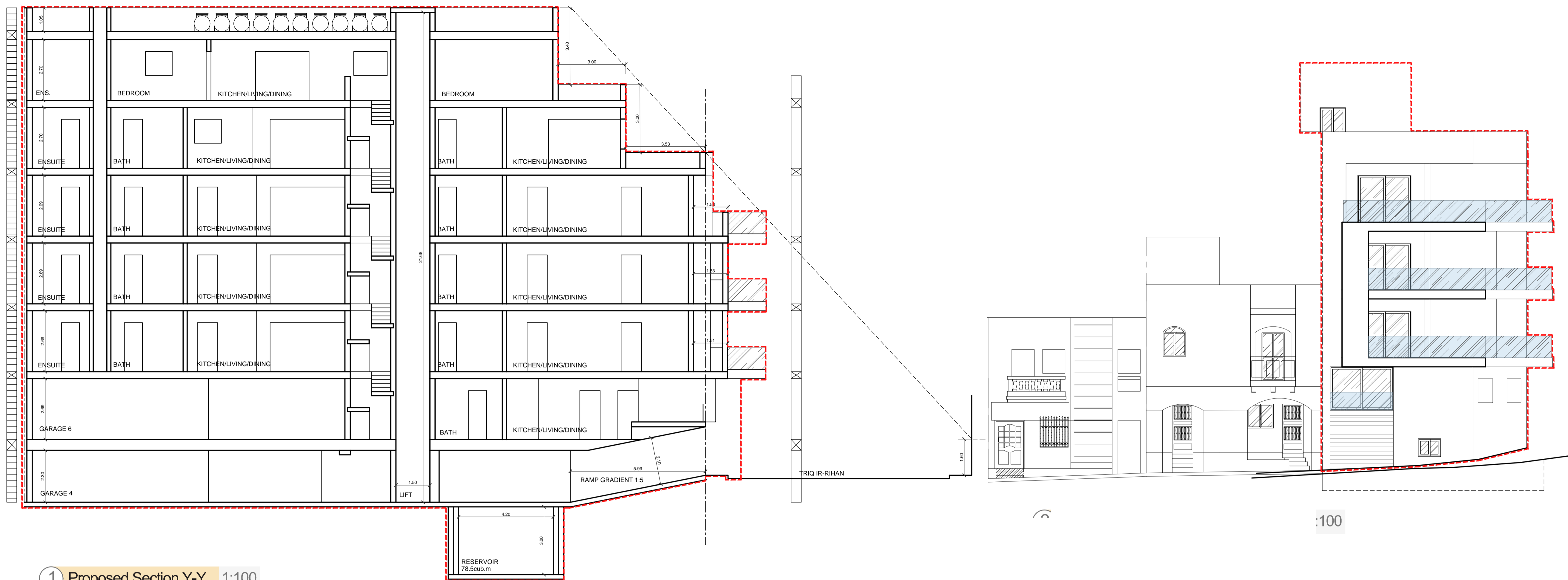
1 Proposed Section Y-Y 1:100
