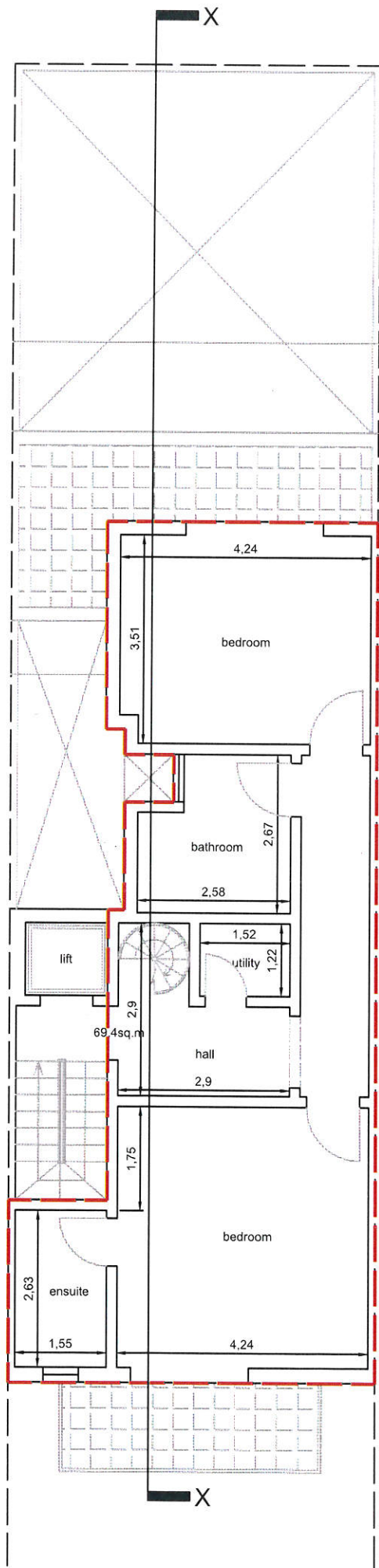
Proposed 5th Floor Plan
