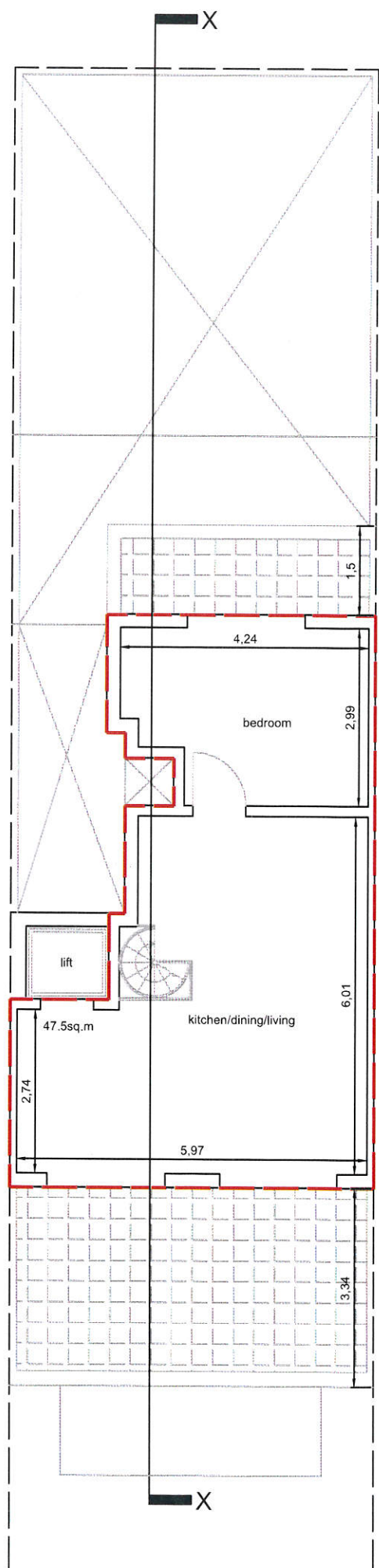
Proposed Receded Floor Plan
