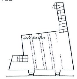
Existing basement plan Scale 1:100
