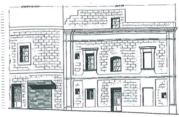
Existing street scape Library St. Scale 1:100
