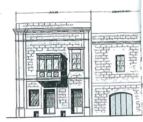
Proposed street scape Vajrapa St. Scale 1:100
