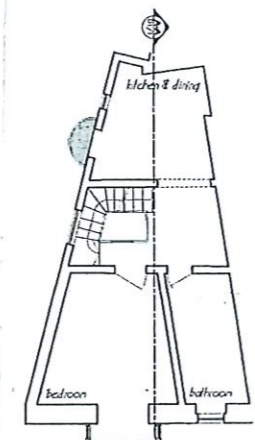
Existing first floor plan Scale 1:100
