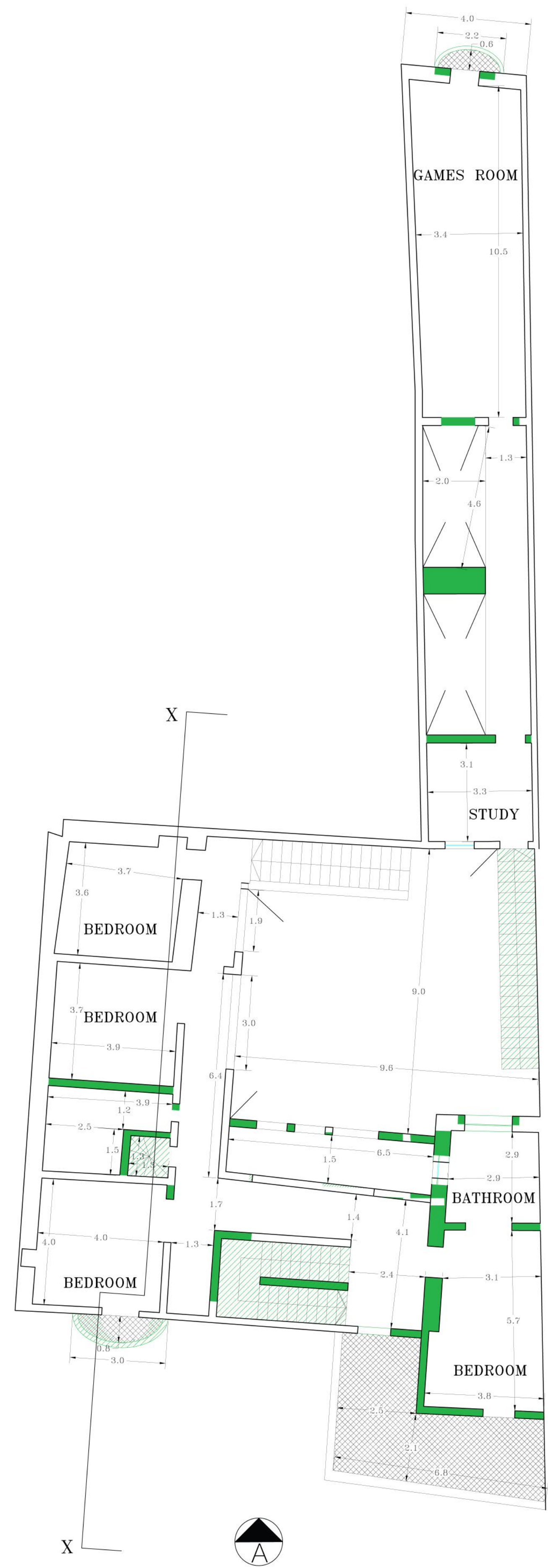
First Floor Approved Plan GROSS FLOOR AREA : 203.5 SQ.M.
