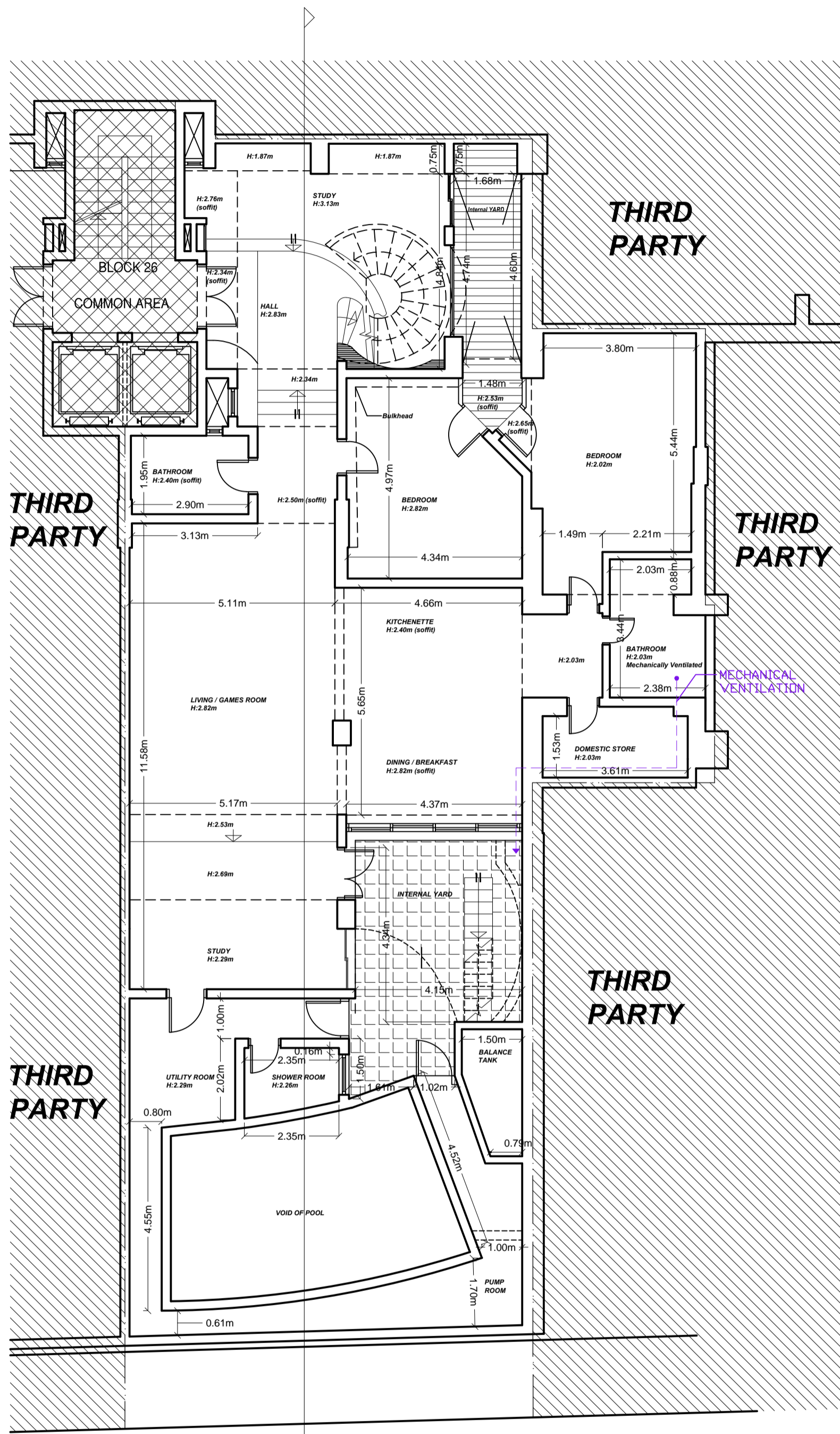
EXISTING DUPLEX LOWER FLOOR PLAN SCALE 1:100
