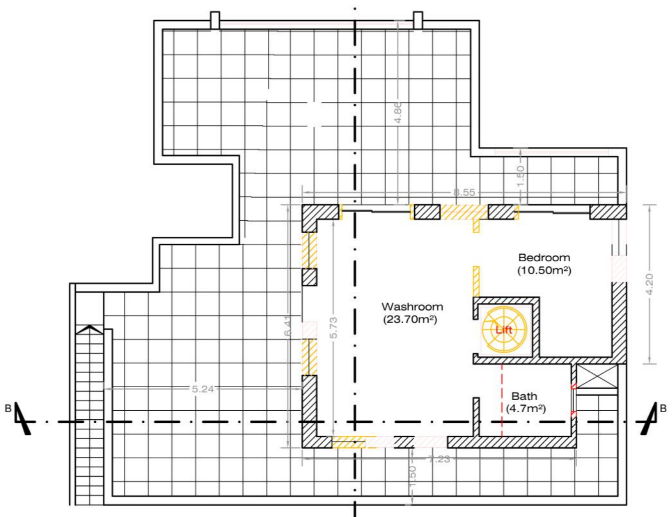
As Approved/Proposed First Floor Plan scale 1:100
