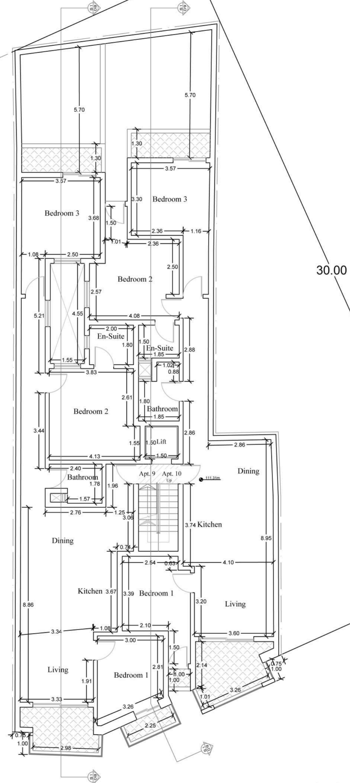
Proposed 5th Floor Level Scale 1:100
