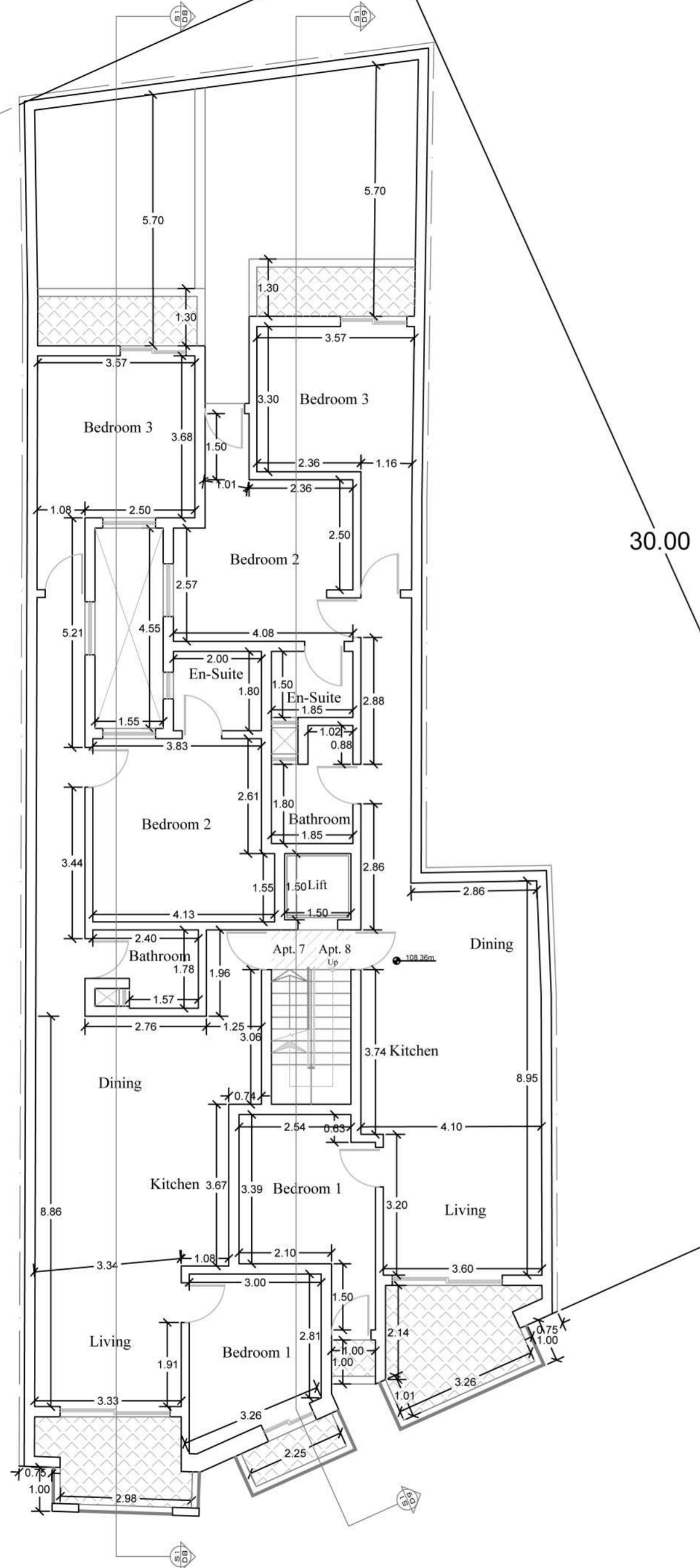
Proposed 4th Floor Level Scale 1:100
