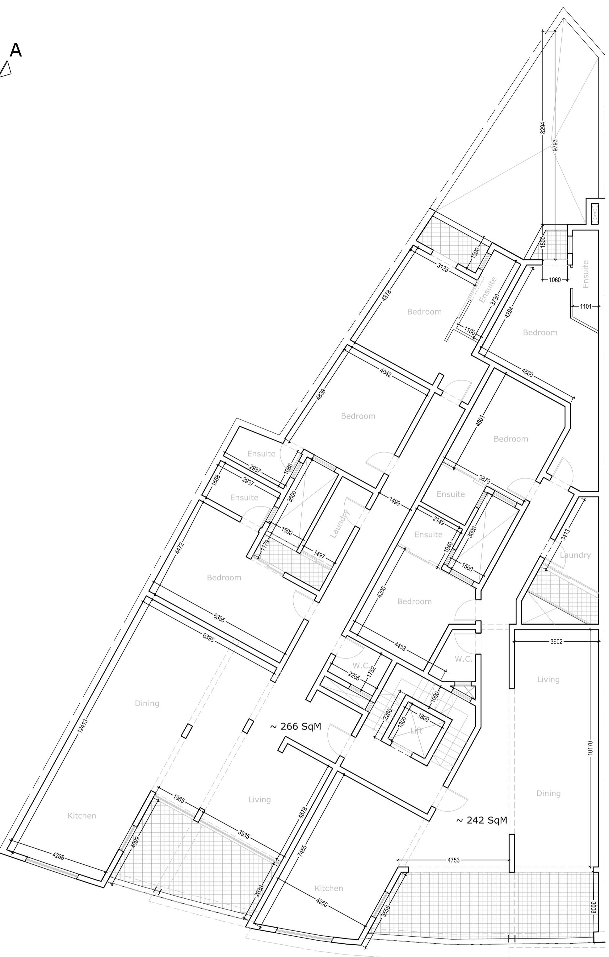
Proposed Second Floor Level Plan
