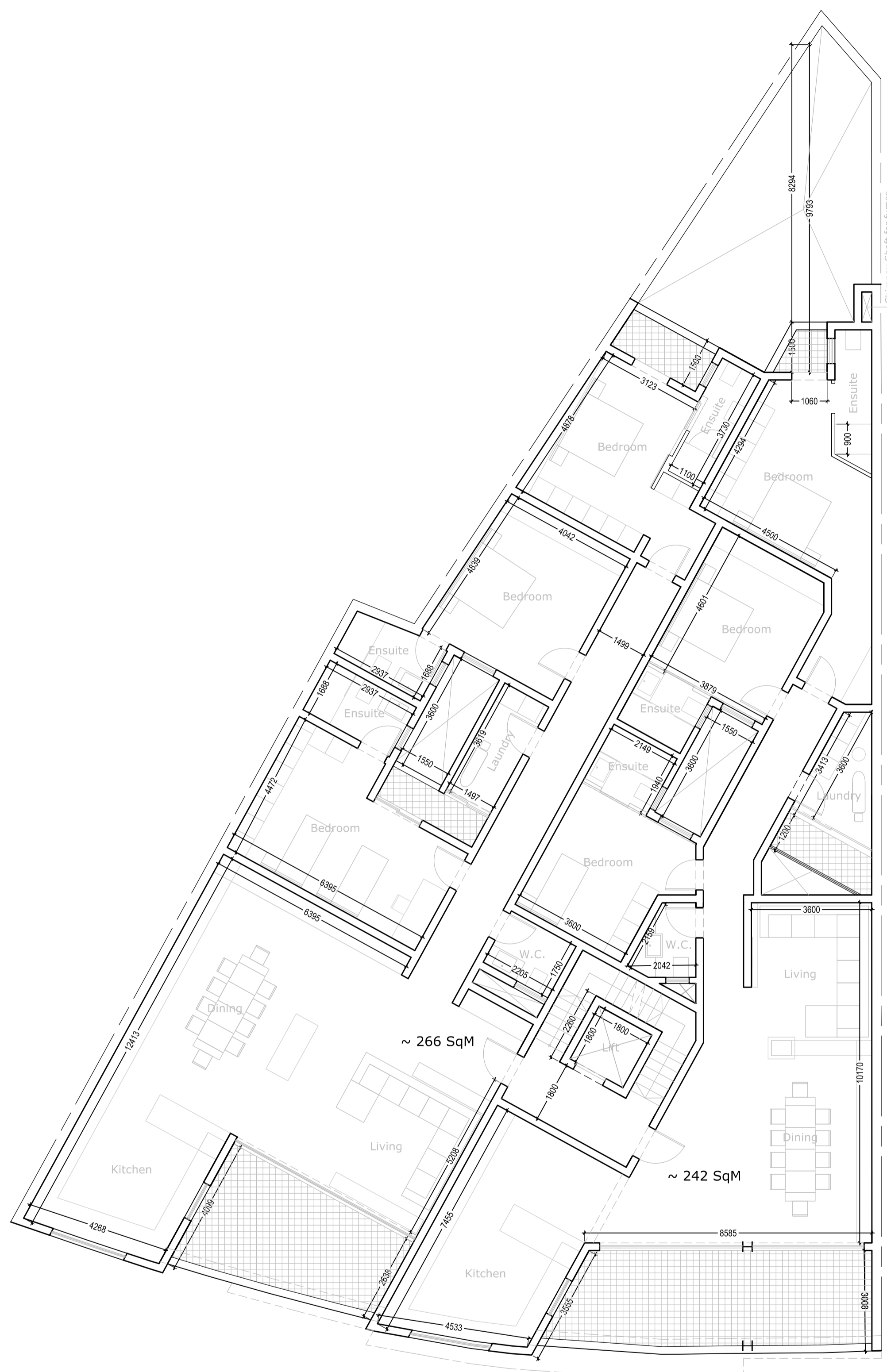
Second Floor Level As Approved in PA/11055/18
