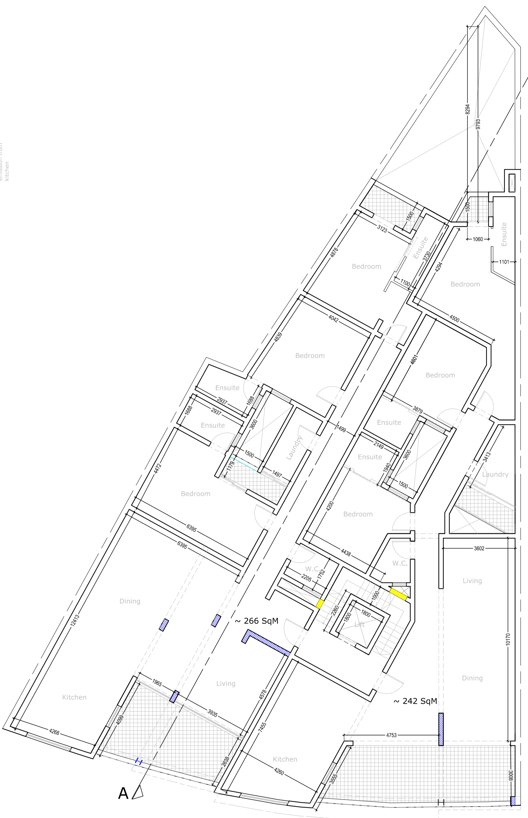
Second Floor Level Plan Proposed Changes Colour Coded
