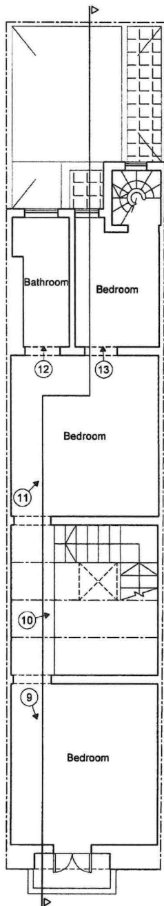
⊙ First Floor Plan 1:100
