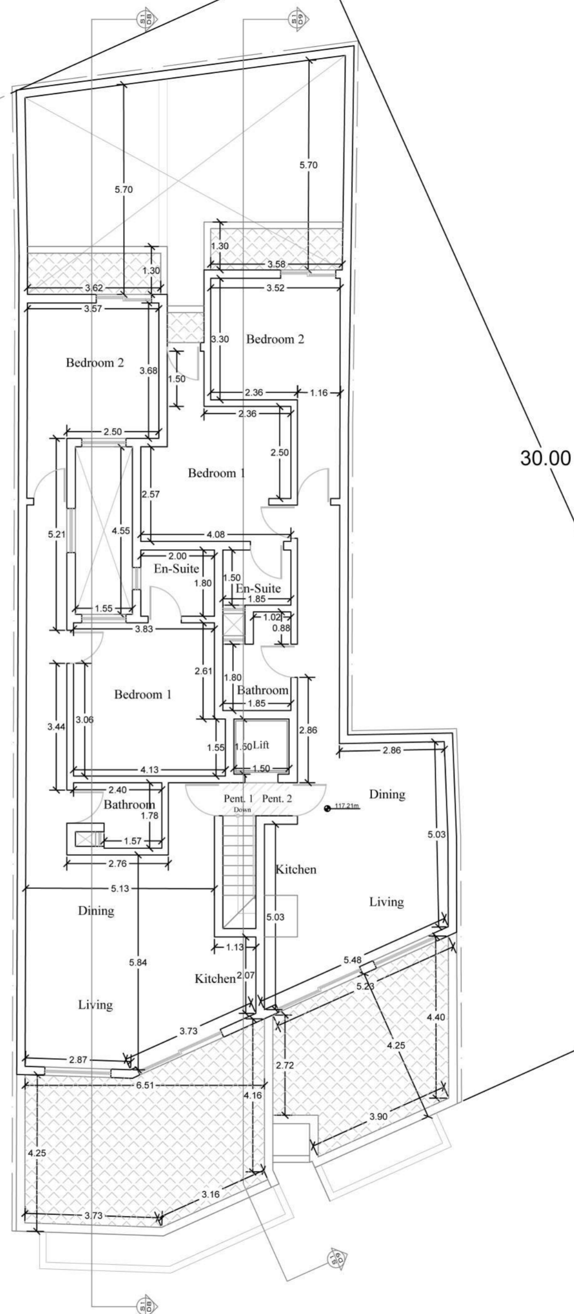
P10 D5 Proposed Receded Floor Level Scale 1:100
