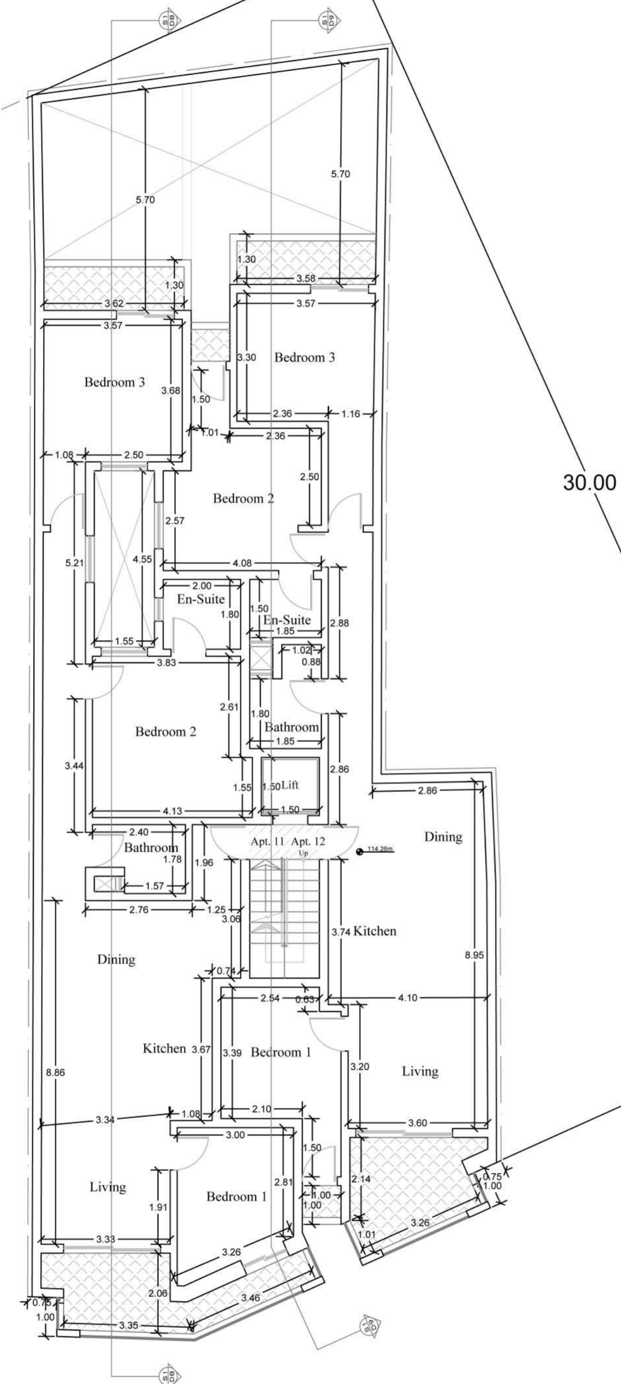
P9 D5 Proposed 6th Floor Level Scale 1:100
