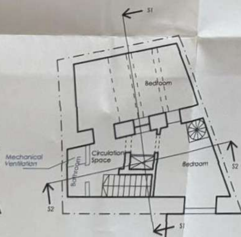
FIRST FLOOR Approved/To Sanction SCALE 1:100
