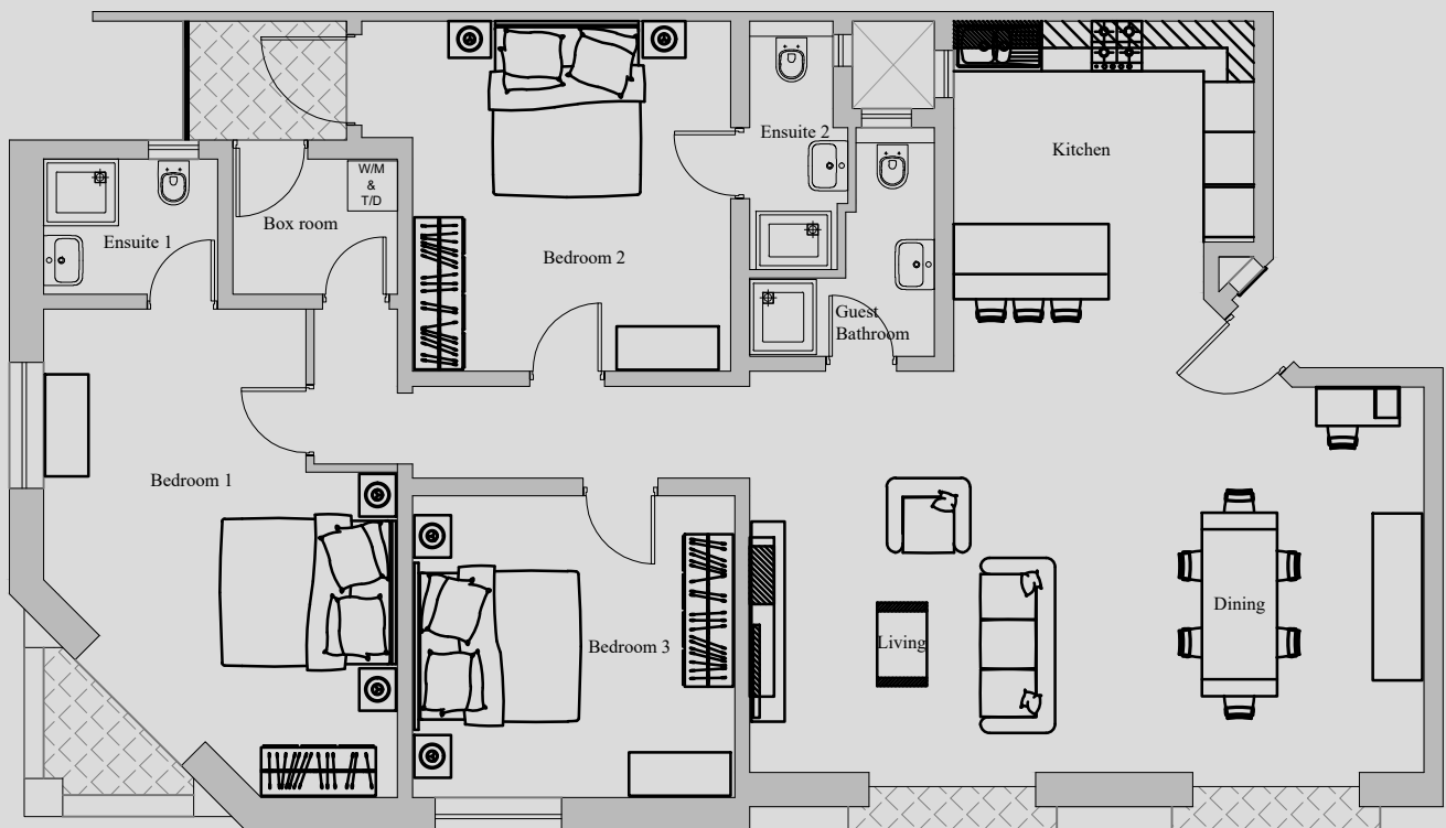
FLOOR PLAN
