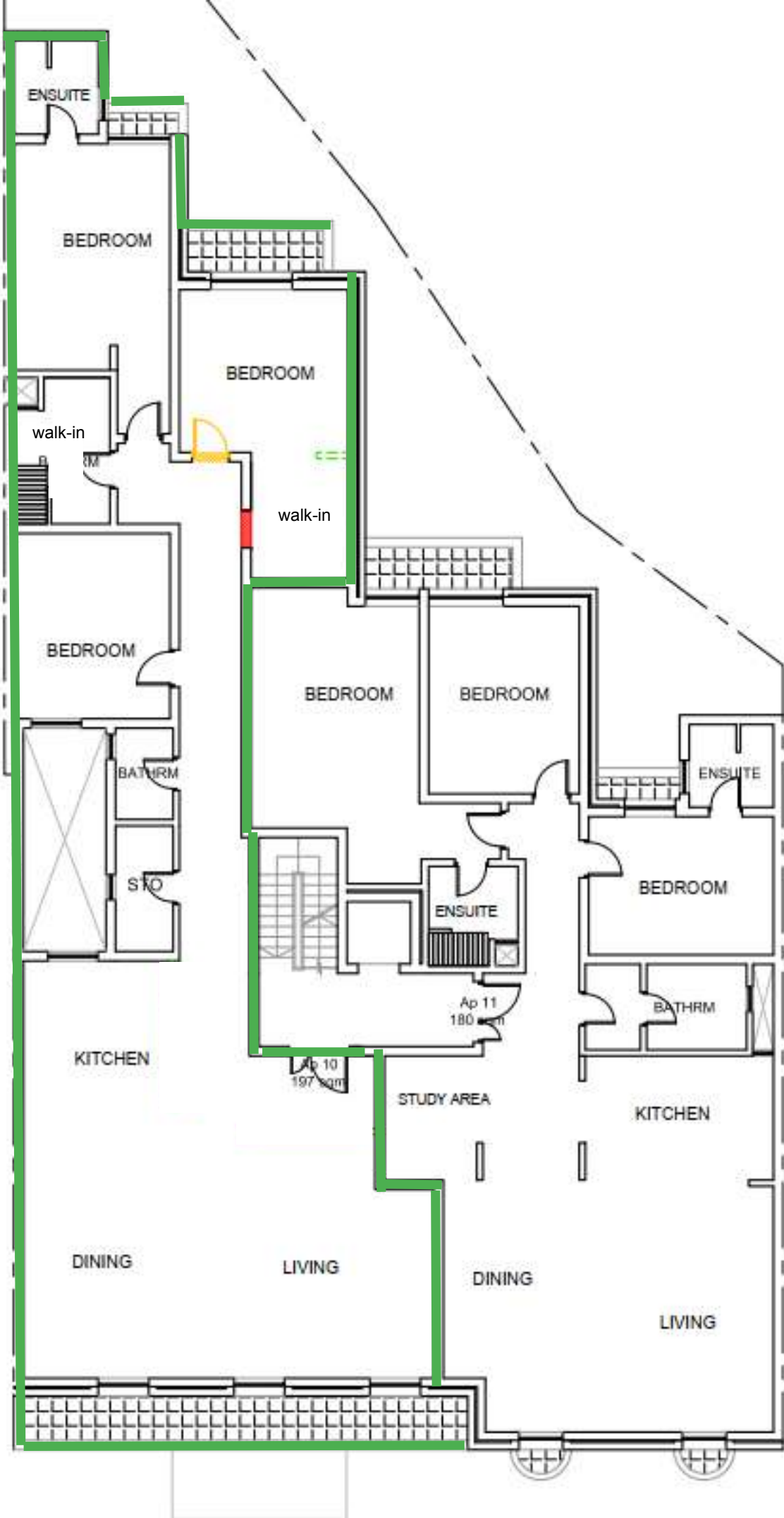
Approved/Proposed Second Floor
