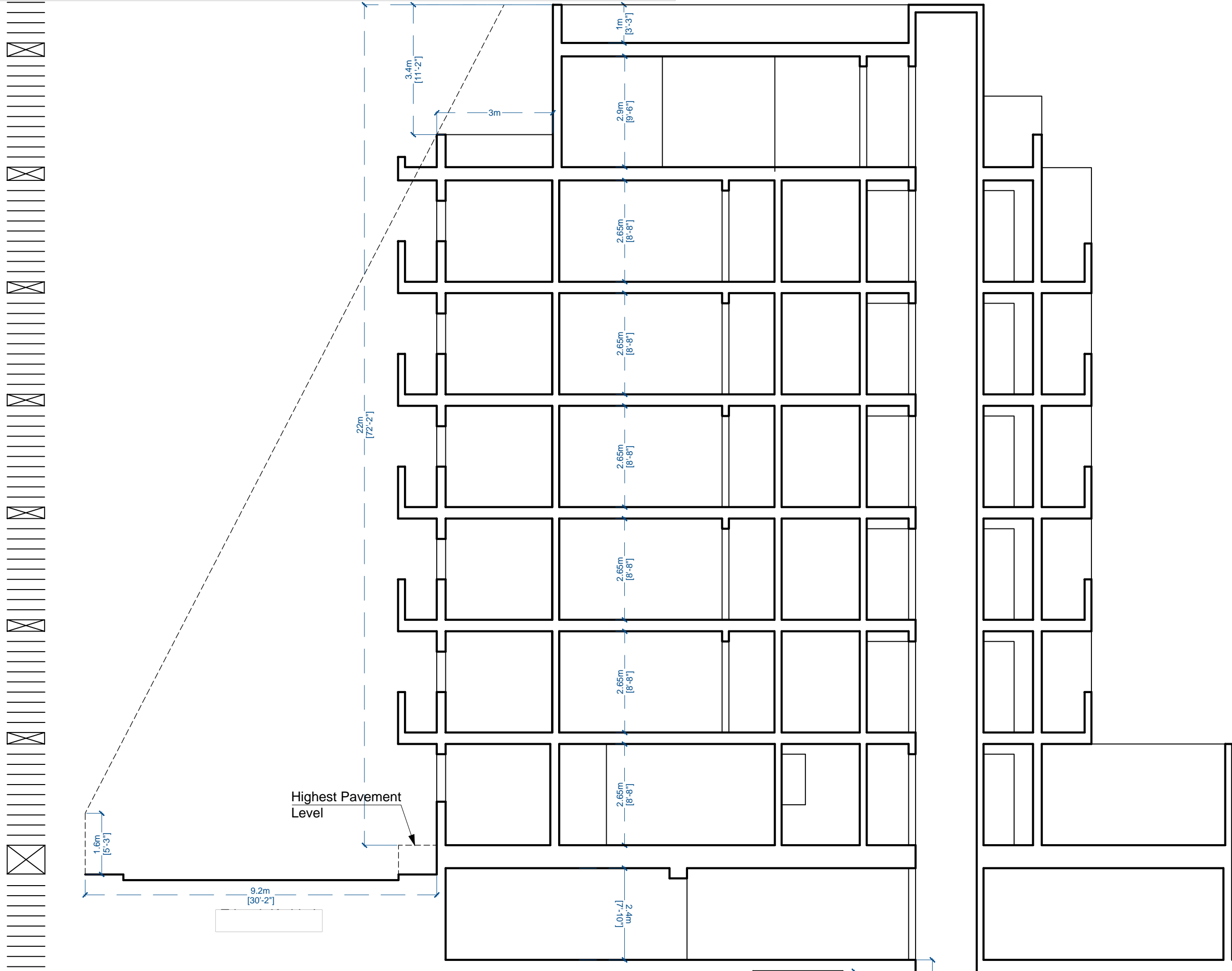
Section BB Proposed Scale 1:100
