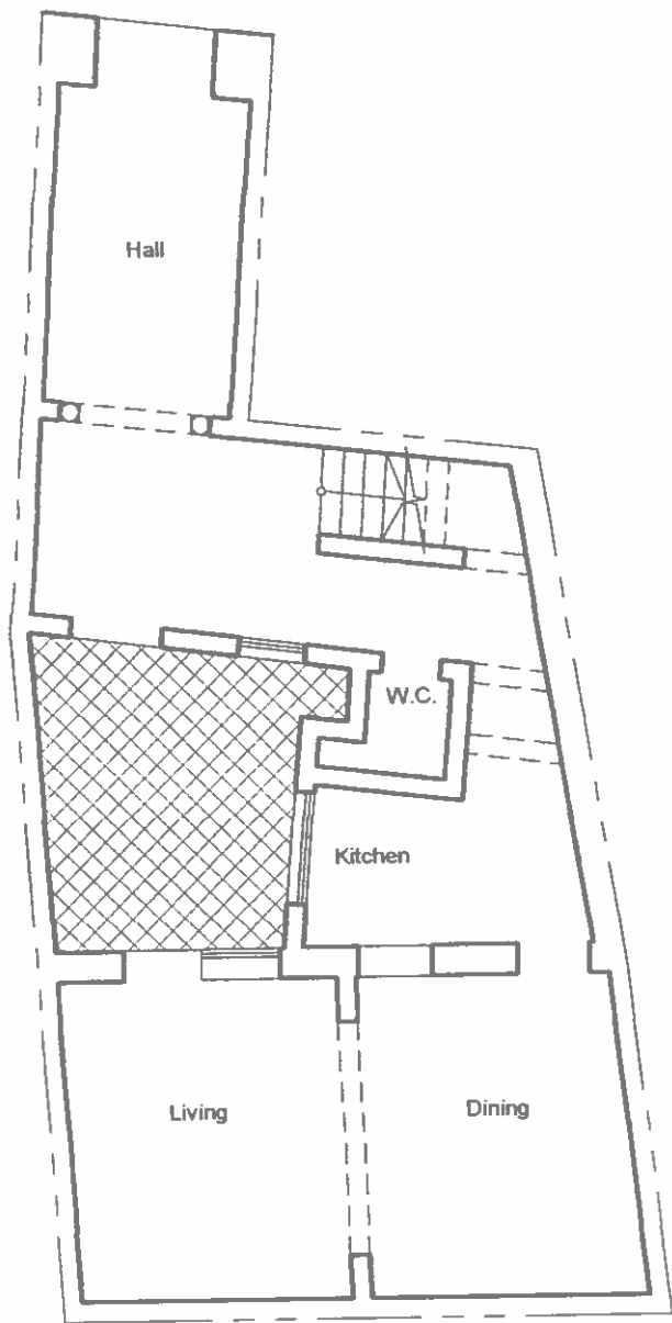
1 EXISTING GROUND FLOOR PLAN SCALE 1:100
